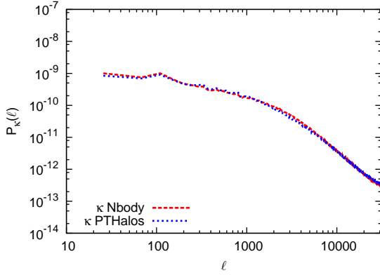
Figure 15. Effective convergence for the N-body halos (red dashed curve) and the 2LPT PTHalos (blue short-dashed curve). Halos are described by a spherical symmetric NFW density profile.
