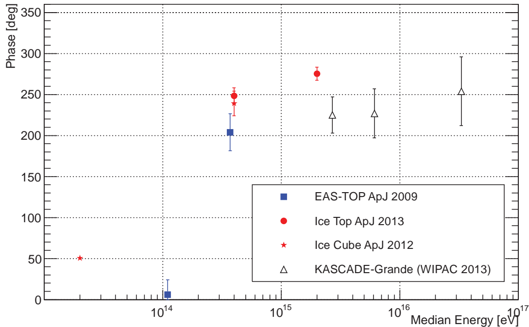
Figure 6. Phases of the first harmonic measured in the 10^{13} - 5 \times 10^{16} eV energy range
