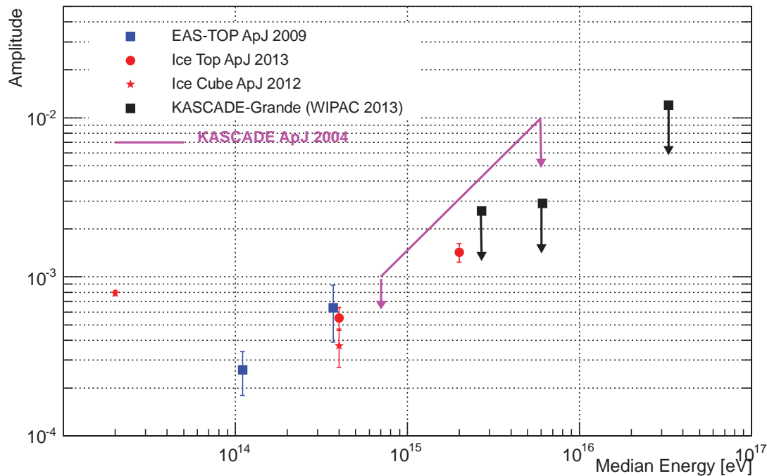
Figure 5. Amplitudes of the first harmonic measured in the 10^{13} - 5 \times 10^{16} eV energy range. The results of the EAS-TOP, IceTop and IceCube experiments are measurement of the first harmonic amplitude, while the KASCADE and KASCADE-Grande ones are upper limits.
