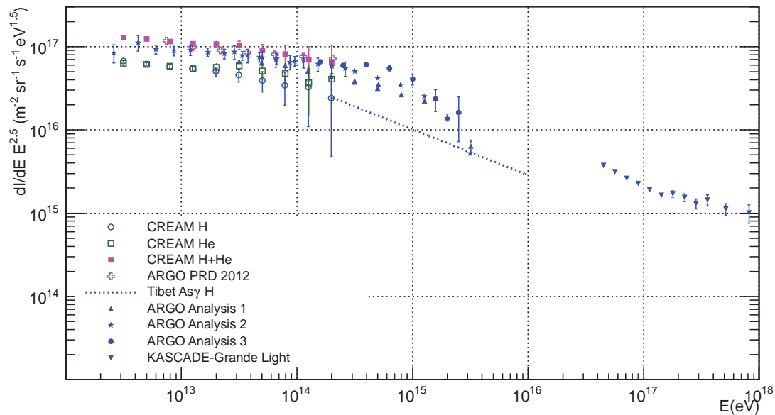
Figure 4. Spectra of the light primaries measured by ARGO-YBJ (the different analysis shown by the collaboration are described in [9]) and KASCADE-Grande. Lower energy direct measurements of the CREAM experiment are shown as a reference. The former KASCADE measurements are not shown in this plot as the light primaries spectrum was shown in a non energy calibrated way [6]
