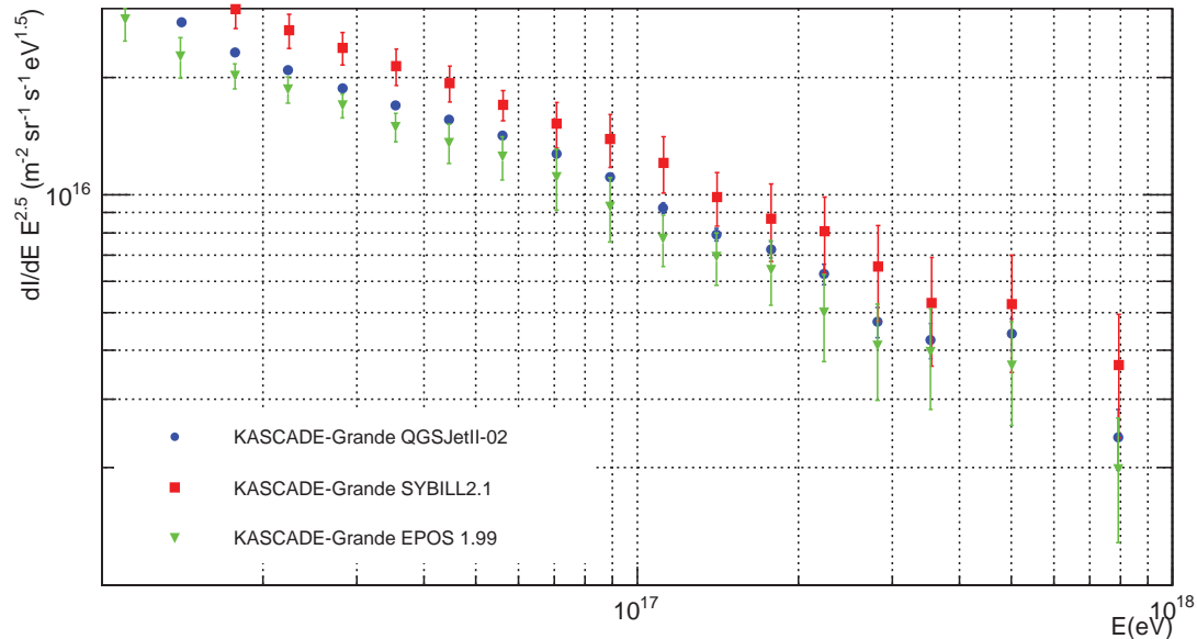
Figure 1. KASCADE-Grande measurements of the all particle energy spectra calibrated by mean of three different hadronic interaction models: QGSJetII-02, Sibyll2.1 and EPOS1.99
