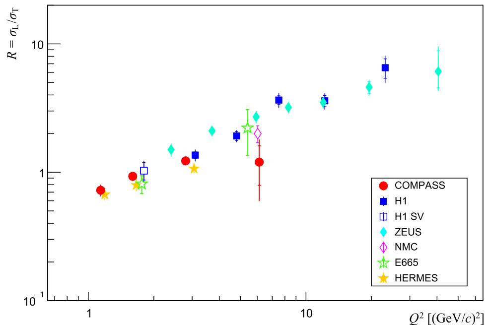
Fig. 13 The ratio R = \sigma_L/\sigma_T as a function of Q^2 . For comparison measurements of exclusive \rho^0 leptonproduction by fixed target experiments (HERMES [23], NMC [24], E665 [25]) and by HERA collider experiments (ZEUS [30], H1 [27], H1 SV [26]) are also shown
