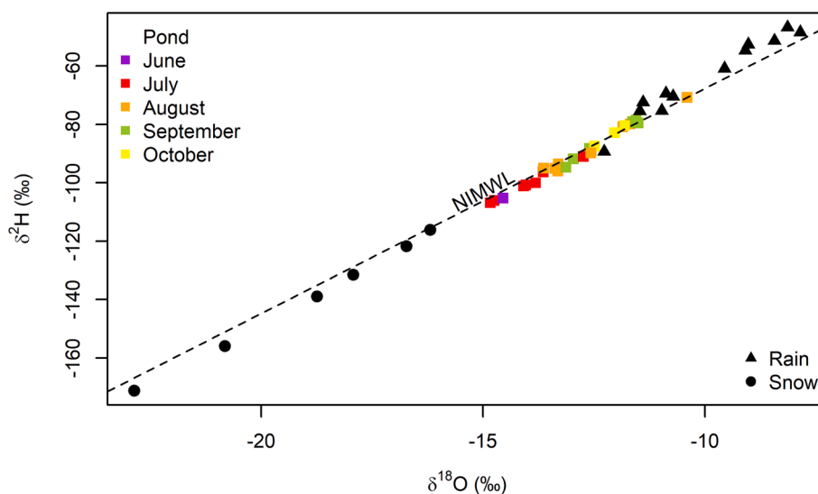
Fig. 3. Dual-plot isotope distribution showing pond, snow and rain data. For pond samples, different colours identify the sampling months (from June to October). NIMWL: Northern Italian Meteoric Water Line.
