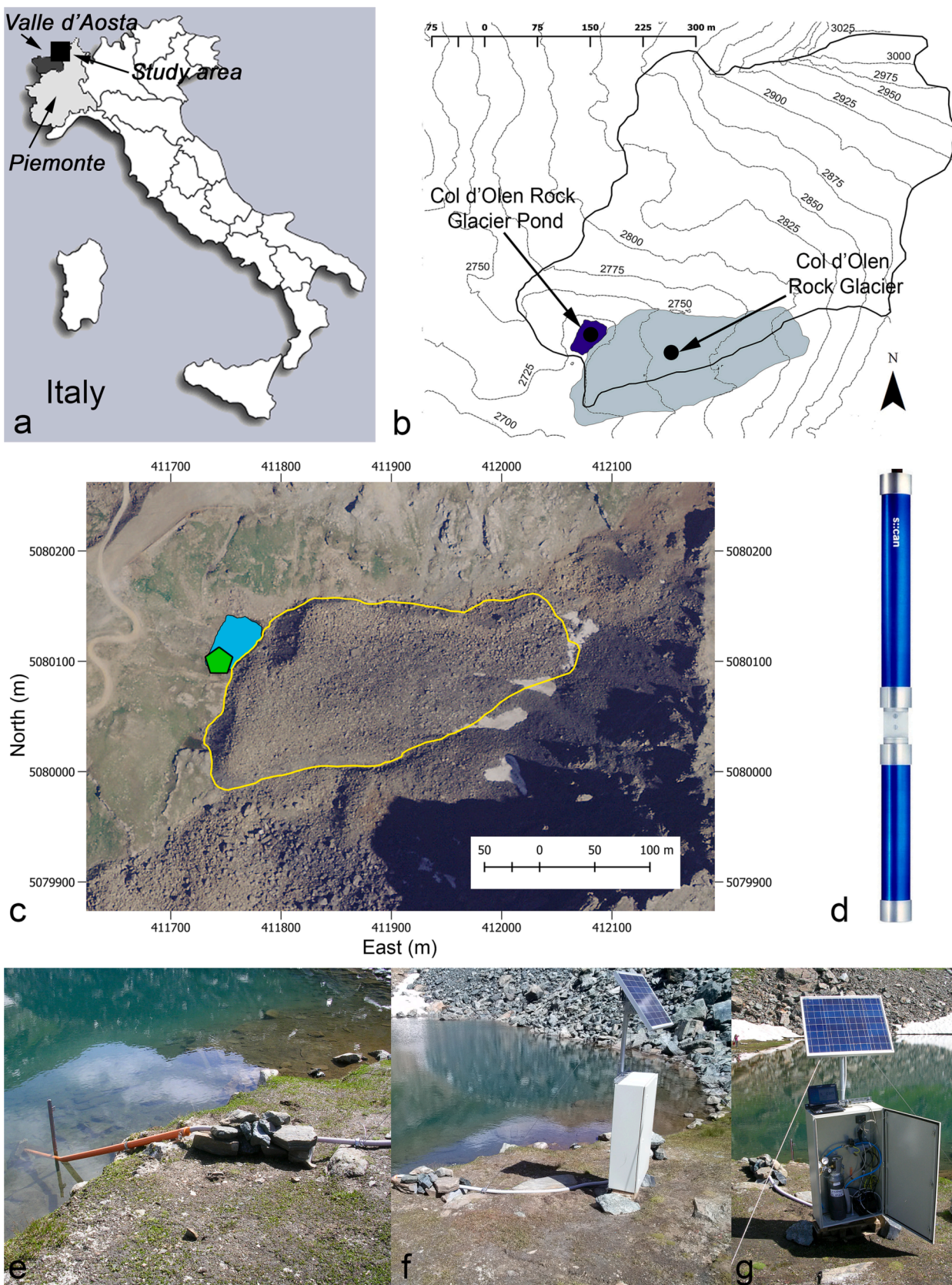
Fig. 1. (a) Location of the study area in Italy. (b) Elevation map of the study area showing the extent of the catchment, the Col d'Olen Rock Glacier, and the Col d'Olen Rock Glacier Pond. (c) Aerial view of the Rock Glacier Pond system and location of the UV-Vis probe (green polygon) on the southern side of the pond (cyan polygon) (aerial image year 2006, coordinate system WGS 84 / UTM zone 32 N). (d) Image of the probe used in this study. Details of the probe installation site: (e) installation in the pond, (f) on-shore installation with electrical and solar panels, and (g) internal view of the electrical panel, with pressurised air system and battery.
