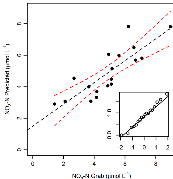
Fig. 4. Scatterplot of grab samples against the values predicted by the linear regression model with confidence levels at 95 % ( n = 18 , r = 0.83 , p < 0.01 ). The inset shows the normal quantile-quantile plot of residuals of the final regression model (x axis: theoretical quantiles; y axis: residual quantiles).
