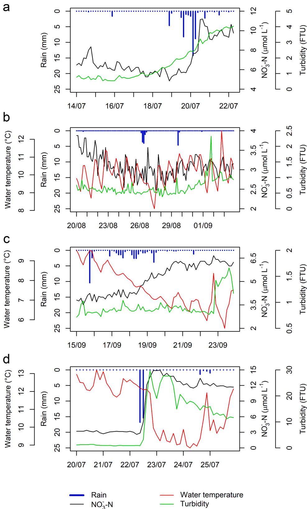
Fig. 6. Three-hourly rain, water temperature (when available), and NO 3 - -N concentrations and turbidity estimated by the probe in four selected periods: (a) 14 – 22 July 2014 (water temperature was not measured in this period), (b) 20 August – 3 September 2014, (c) 15 – 23 September 2014, and (d) 20 – 25 July 2015.
