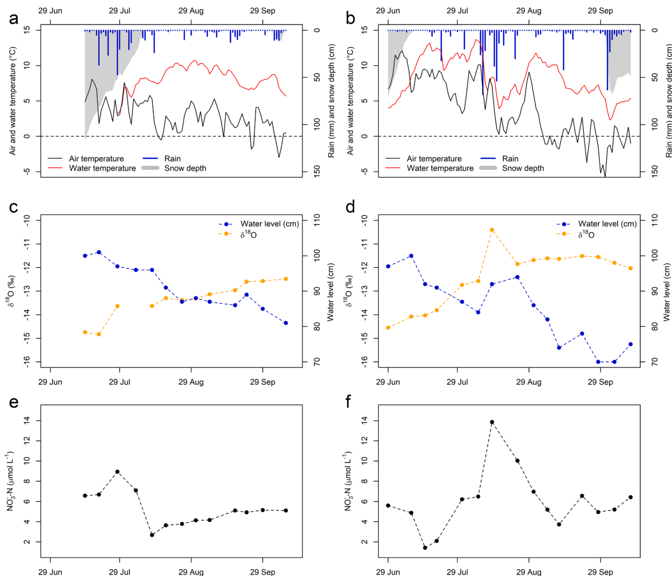
Fig. 2. Daily air temperature, water temperature, rain, and snow depth in (a) 2014 and (b) 2015. Water level and \delta^{18}\text{O} values in grab samples in (c) 2014 and (d) 2015 (only \delta^{18}\text{O} is shown given the high correlation with \delta^2\text{H} ). \text{NO}_3^- \text{-N} concentrations in grab samples in (e) 2014 and (f) 2015.
