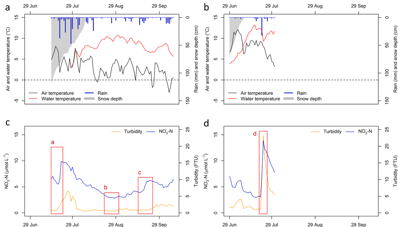
Fig. 5. Daily air temperature, water temperature, rain, and snow depth in (a) 2014 and (b) 2015 (meteorological conditions are shown in Fig. 2 and here to enhance the interpretation of the \text{NO}_3^- -N and turbidity variations measured by the probe). Daily \text{NO}_3^- -N concentrations and turbidity estimated by the probe in (c) 2014 and (d) 2015. Red windows in panels c and d refer to panels a–d in Fig. 6.
