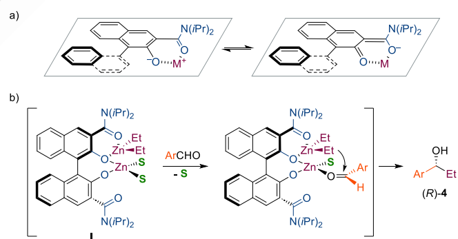
Figure 4. a) π-conjugated, flat metal-chelated conformation of I and b) proposed transition state model for the asymmetric alkylation of aldehydes catalysed by BINOL-Zn(II) dinuclear complex I . [15]
