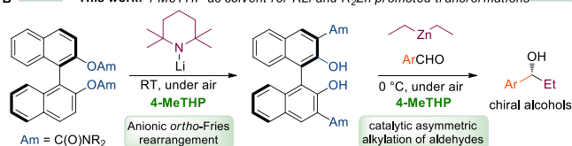
Figure 1. a) State-of-the-art of the employment of 4-methyltetrahydropyran (4-MeTHP) as reaction media in synthetic transformations promoted by organometallic reagents, [10–12] and b) aim of this work.
