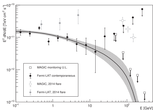
Figure 3. Comparison of the MAGIC SED upper limits (black empty squares) with the extrapolation (black line and shaded region) of the Fermi -LAT spectrum (black filled circles). The extrapolation assumes a power-law behaviour and an extragalactic background light (EBL) absorption following Domínguez et al. (2011) model. For comparison, the Fermi -LAT and MAGIC SED during the 2014 flare (Ahnén et al. 2016) are shown with grey markers.
