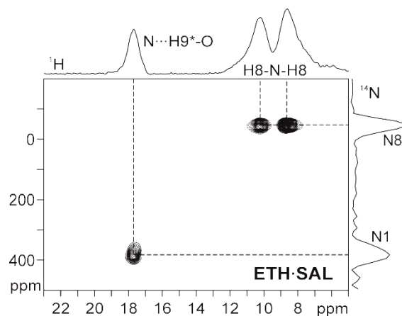
Figure 4. 2D ^1\text{H}\{-^{14}\text{N}\} D-HMQC spectra ( ^1\text{H} = 600.1 MHz, ^{14}\text{N} = 43.4 MHz, \nu_{\text{R}} = 70 kHz) of \text{ETH}^+\text{SAL}^- (top) and \text{ETH}\cdot\text{SAL} (bottom).
