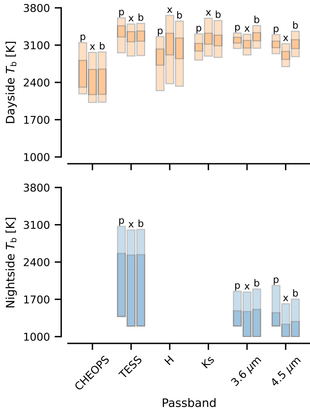
Fig. C.1. Day- and nightside brightness temperatures estimated from the flux ratios using the p) physical-physical, x) blackbody-physical, and b) blackbody-blackbody approaches. The shading marks the 68% and 99.7% central posterior intervals.
