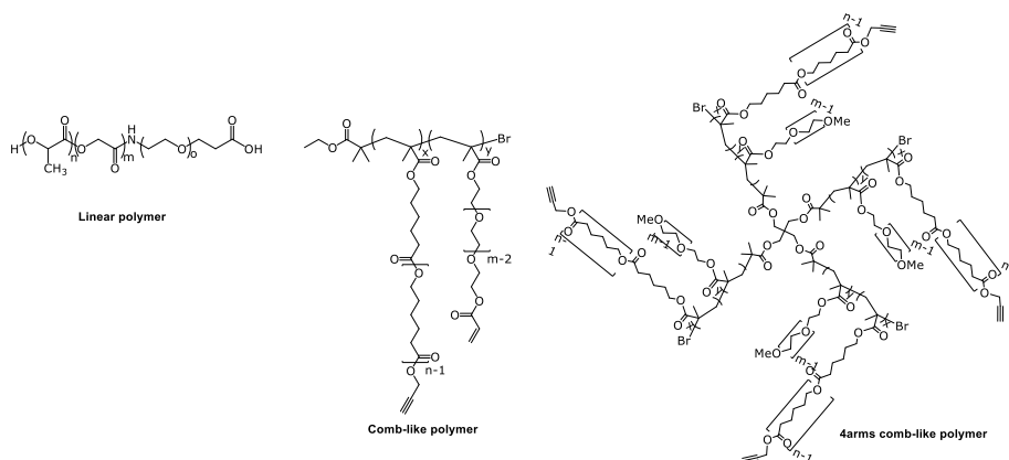
Figure 1: Polymers structure.
