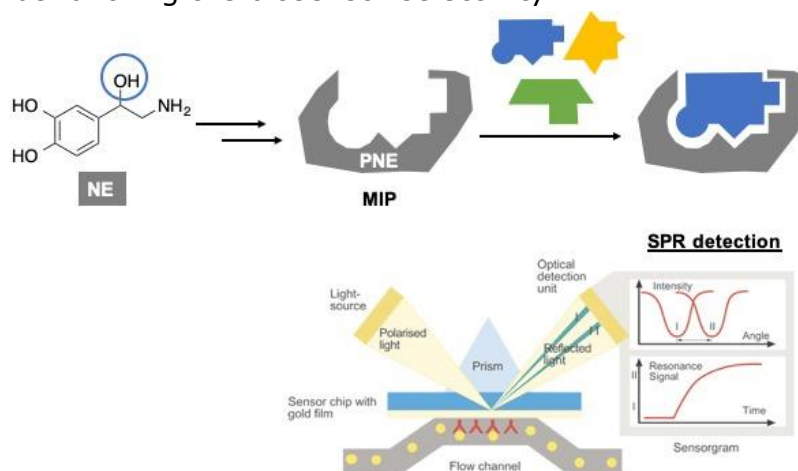
Figure 1: NE as functional monomer for MIP-based biosensors and SPR detection.
