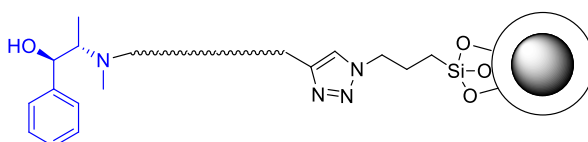
Figure 1: Ephedrine-based nanocatalyst.
