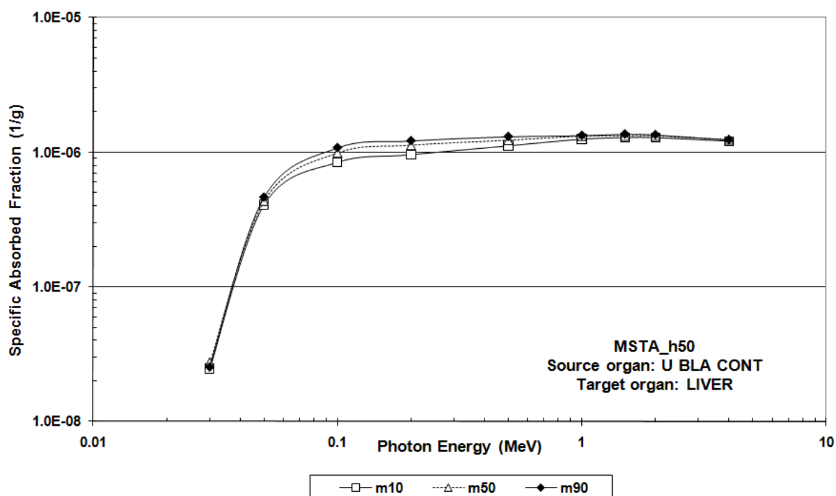
Figure 17. SAF(liver←UBC) as function of the emitted photon energy in the anthropometric phantoms MSTA_h50 for 10 th , 50 th and 90 th mass percentiles.
