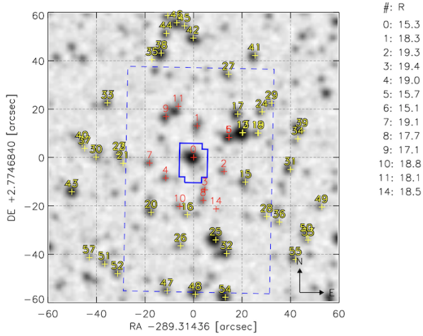
Figure 5. DSS image of CoRoT-35 with the photometric mask overlaid. North is up, and east is on the right.
