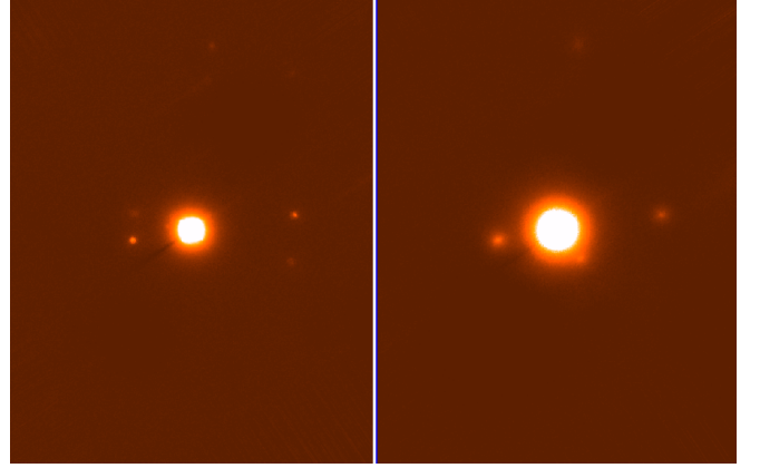
Figure 11. Images taken with the AO-system PISCES at the LBT in the K (left) and in the J-band (right). The size of the image is only about 6 \times 8'' , north is up and east is left. Two previously unknown stars at distances of 1^{\circ}96 \pm 0^{\circ}04 and 3^{\circ}46 \pm 0^{\circ}04 are visible. The orientation is as in Fig. 9.
