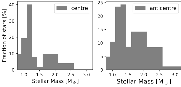
Figure 1. Mass distribution of main-sequence stars in the CoRoT fields. left - Galactic centre fields from photometric classification based on Exodad (Deleuil et al. 2009; Damiani et al. 2016), right - Galactic anticentre fields based on data from (Sebastian et al. 2012; Guenther et al. 2012).
