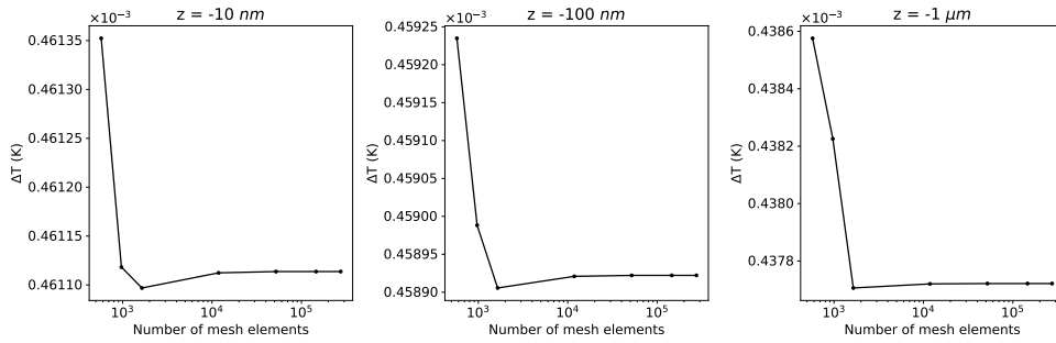
Figure S1: Temperature at r = 0 and at three different depths in the stationary scenario as a function of the different number of mesh elements. The largest number of elements was chosen in order to obtain element sizes comparable to the length scale under investigation.
