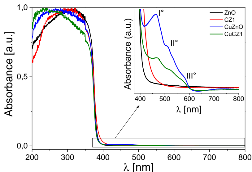
Figure 2. UV- vis analysis (Absorbance Kubelka-Munk transformed diffuse reflectance spectra) of: ZnO (black line), CZ1 (red line), CuZnO (blue line), CuCZ1 (green line).
