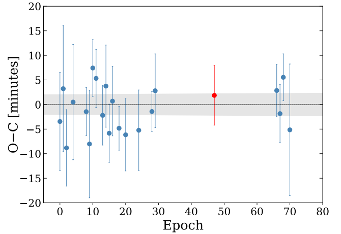
Figure 8. Observed minus Calculated diagram of the transit mid-times of TOI-220 b . Blue symbols correspond to TESS transits while the red symbol correspond to the second LCOGT transit observation. The shaded region represents the projected 1\sigma uncertainties of ephemeris equation of TOI-220 b (Sect. 3.4).
