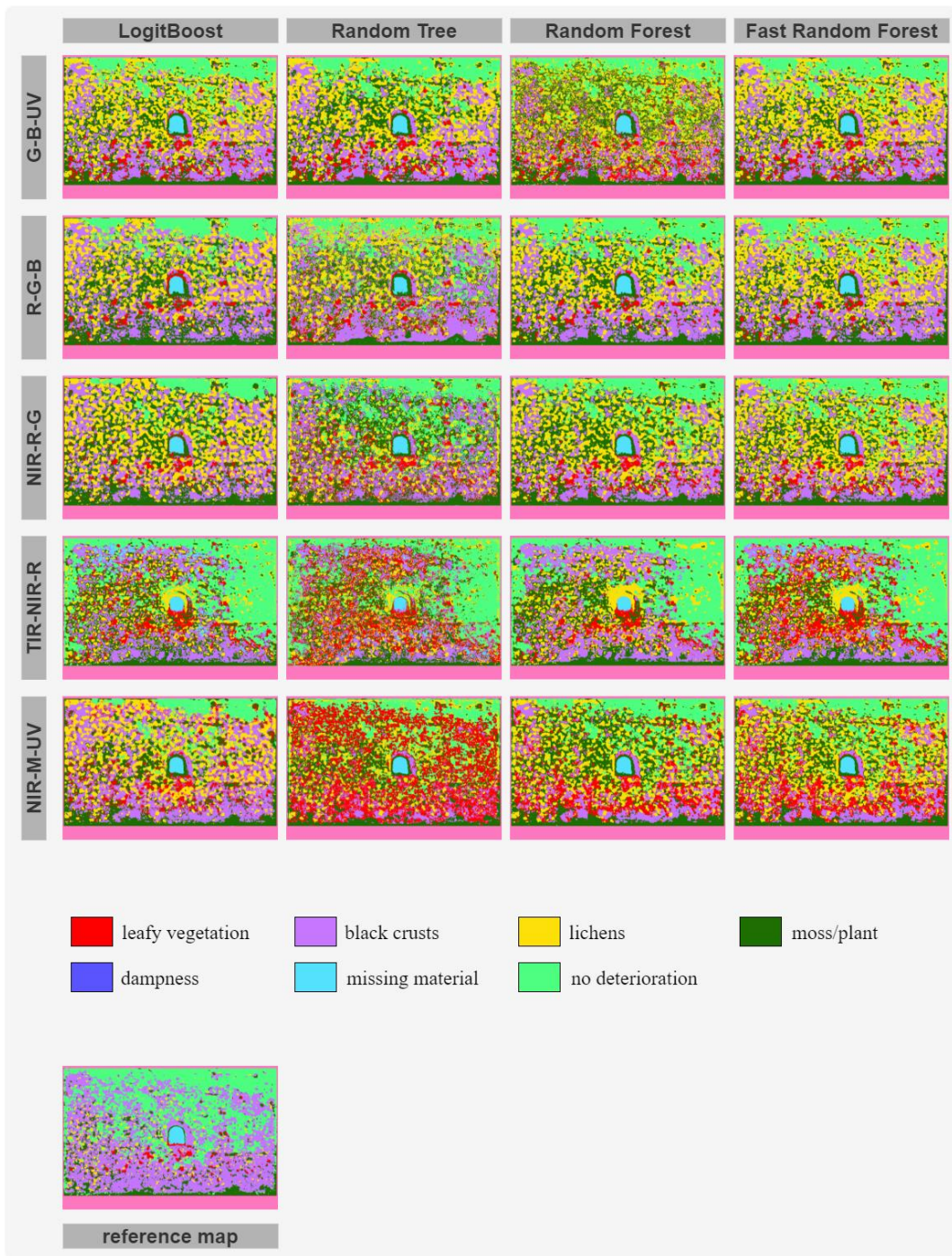
Figure 4.6. Thematic deterioration mapping of façade A, Fort of Karababa.
