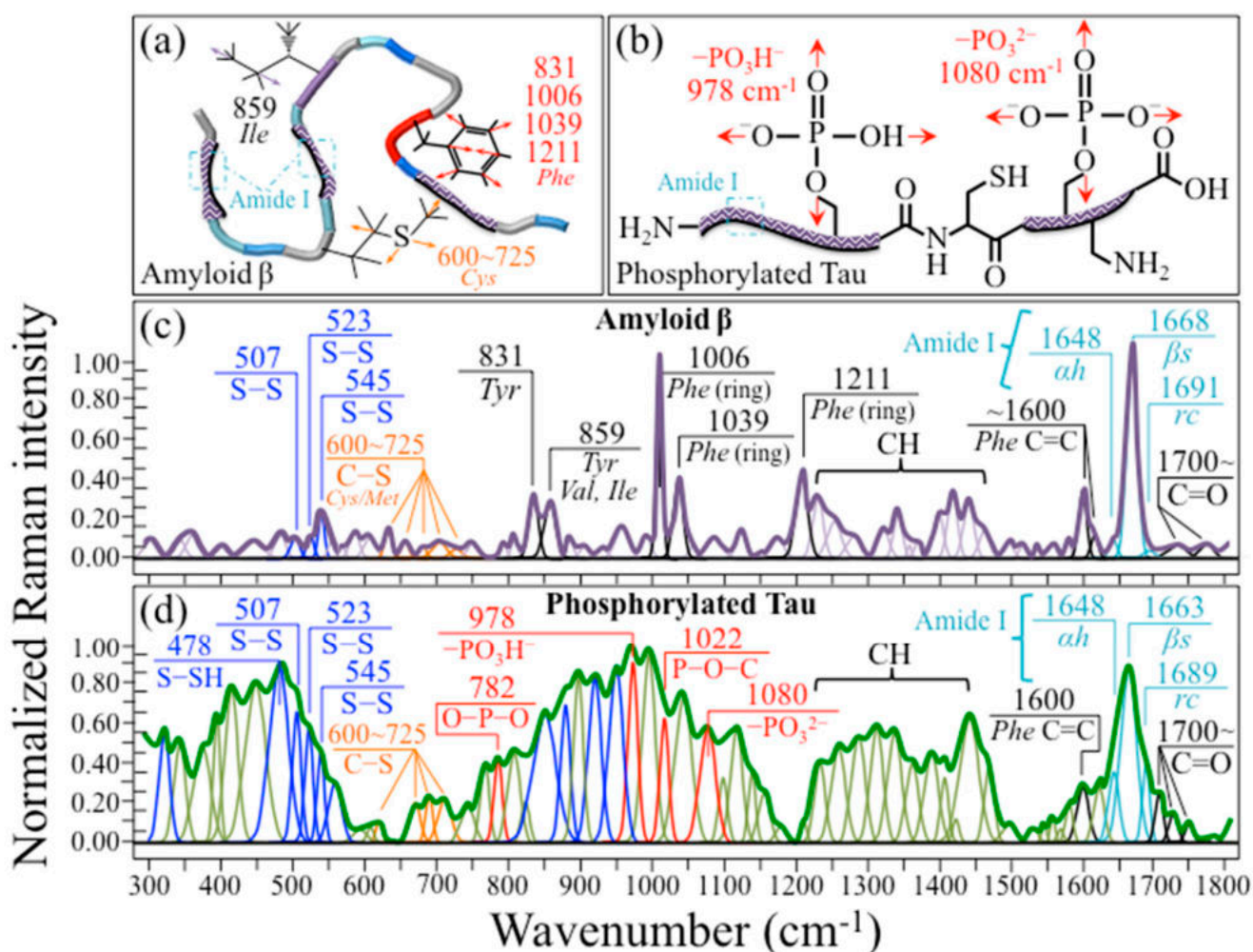
Figure 6. Schematic drafts of (a) an A\beta fibril and (b) a phosphorylated Tau filament; (c,d) their average and deconvoluted Raman spectra, respectively, as recorded in the wavenumber interval 300–1800 \text{cm}^{-1} . Band assignments are given in the figure and described in the text. The abbreviations Cys, Met, Phe, Tyr, Val, and Ile represent cysteine, methionine, tyrosine, valine, and isoleucine amino acid residues, respectively. The abbreviations \alpha h, \beta s, and rc represent \alpha -helix, \beta -sheet, and random coil, respectively. Colored arrows represent the vibrations of the molecules in the respective insets.
