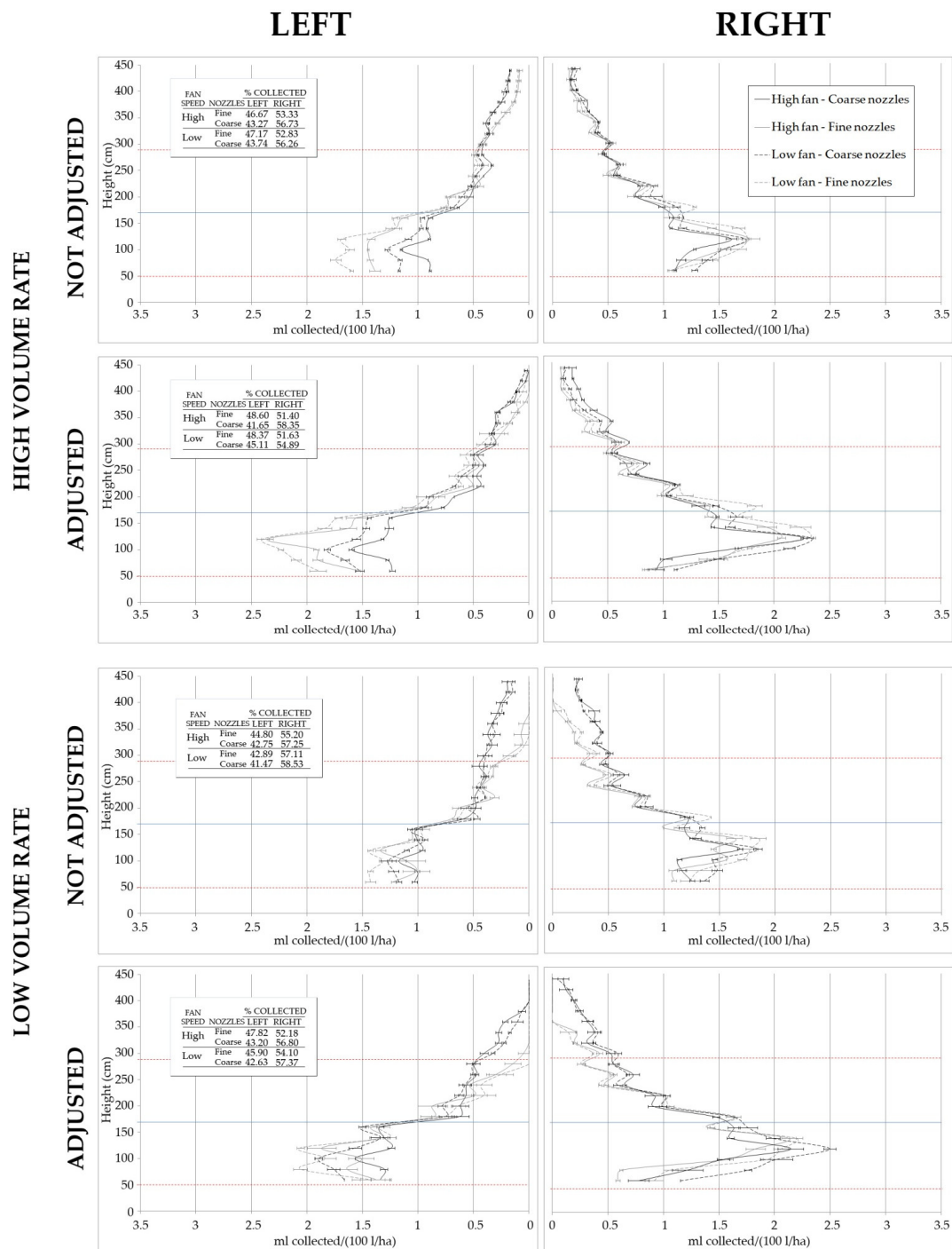
Figure 9. Vertical spray profiles showing the normalized volume collected by the patternator (mL/(100 L/ha) (mean ± SE) at different heights above the ground (m), for the applications with the C1 sprayer . The percentage collected on each side of the sprayer respect to the total volume collected for each configuration is shown. The red dashed lines represent the upper and the lower limit of the canopy, and the blue line its middle height.
