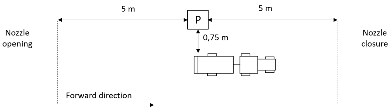
Figure 7. General scheme of the tests (P: Patternator).
