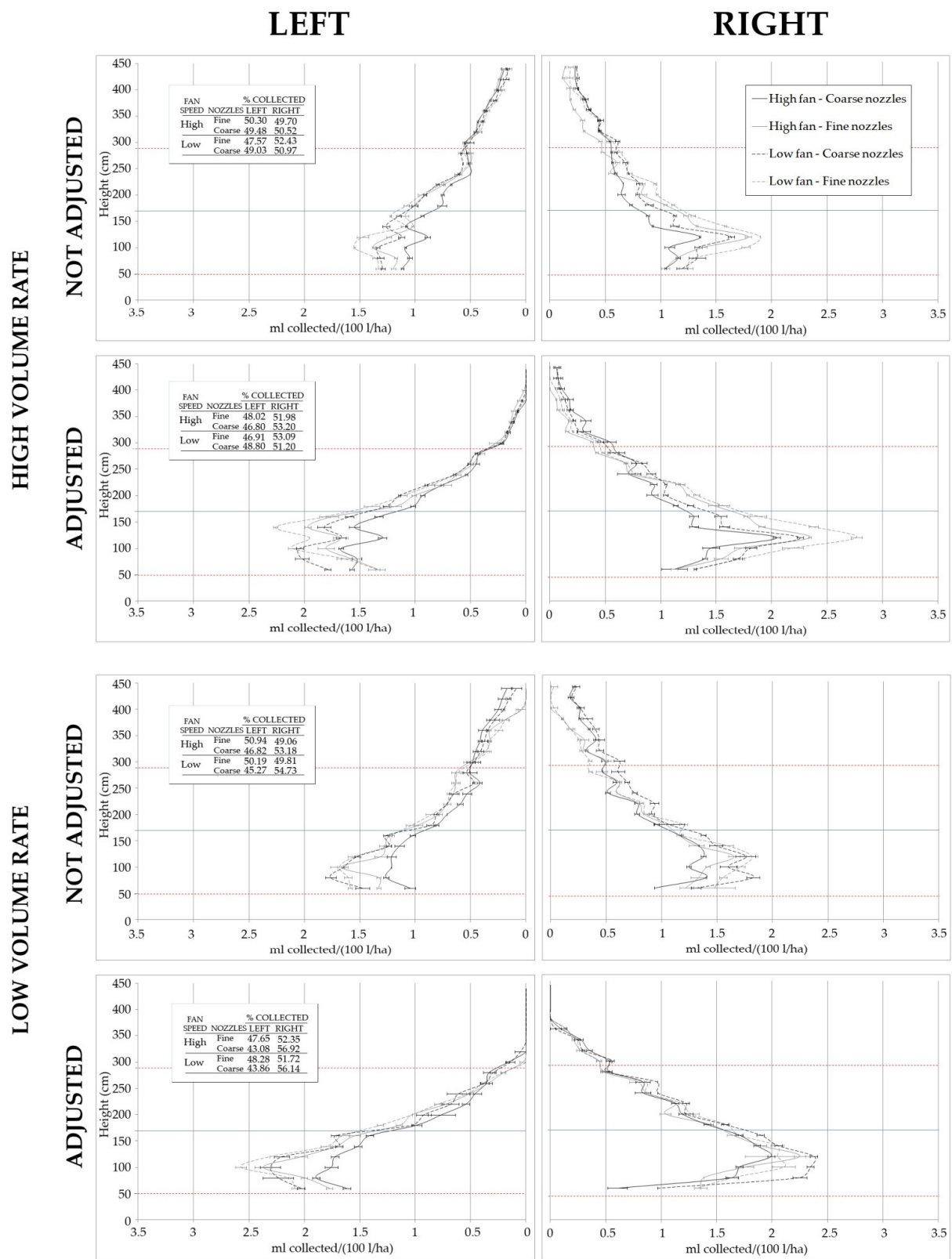
Figure 10. Vertical spray profiles showing the normalized volume collected by the patternator (mL/(100 L/ha) (mean ± SE) at different heights above the ground (m), for the applications with the C2 sprayer . The percentage collected on each side of the sprayer respect to the total volume collected for each configuration is shown. The red dashed lines represent the upper and the lower limit of the canopy, and the blue line its middle height.
