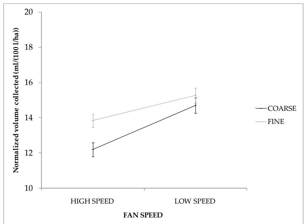
Figure 22. Nozzle type \times Fan speed interaction effect on the normalized volume collected in the canopy zone (mean \pm SE) with the C2 sprayer.
