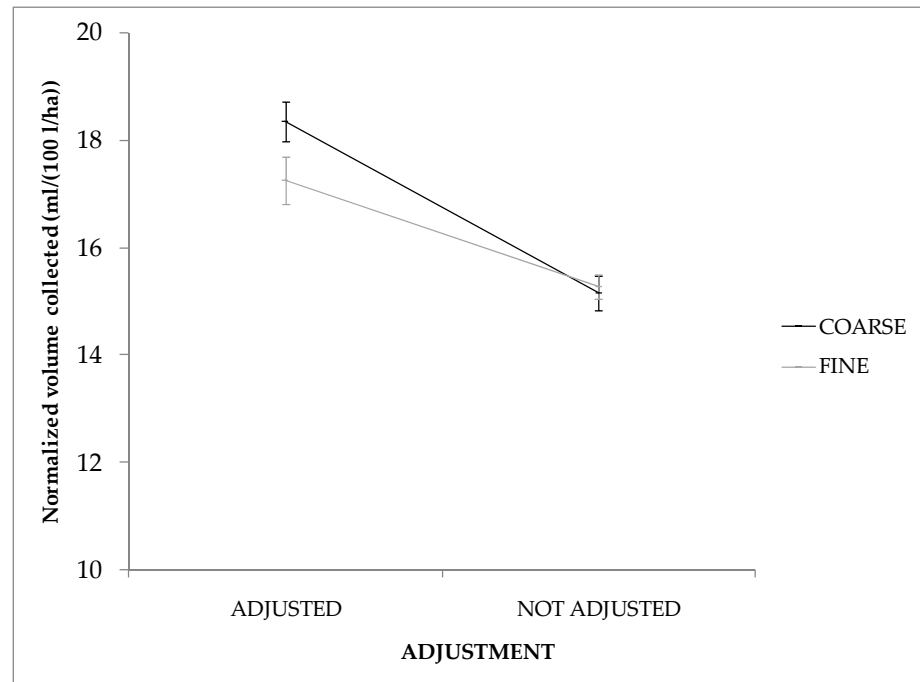
Figure 11. Adjustment \times Nozzle type interaction effect on the normalized volume collected in the canopy zone (mean \pm SE) with the T sprayer.
