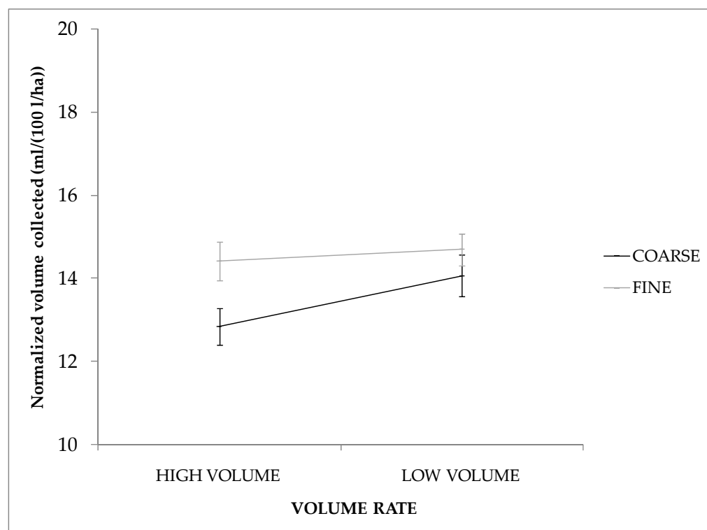
Figure 23. Nozzle type x Volume rate interaction effect on the normalized volume collected in the canopy zone (mean \pm SE) with the C2 sprayer.
