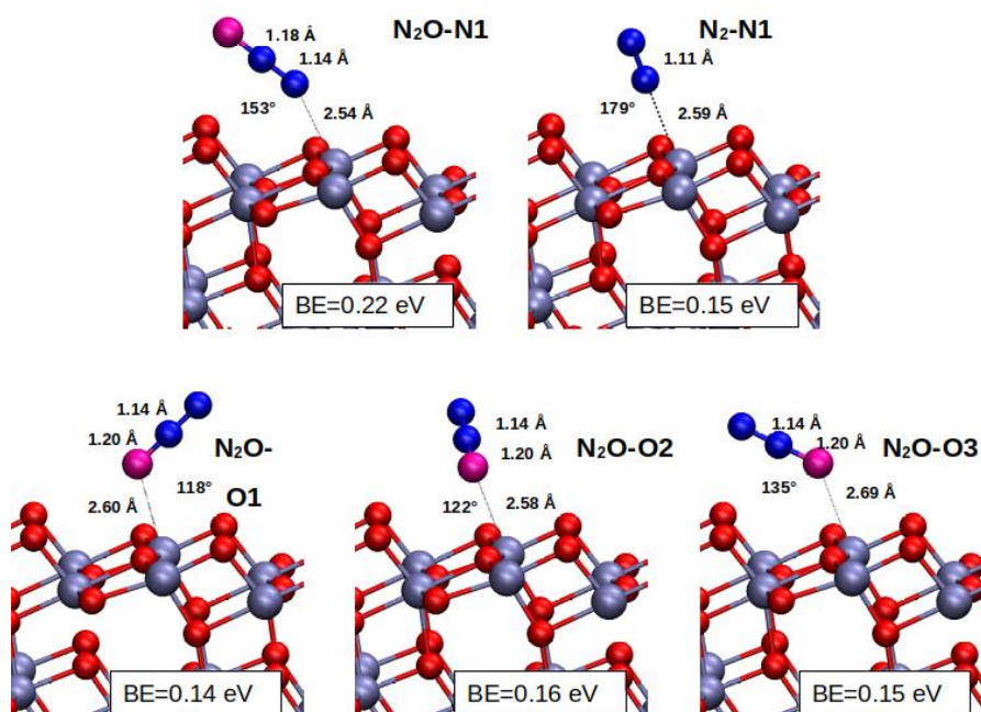
Figure 5. Different possible surface configurations for N_2O adsorption at \theta = 0.25 from the N-end ( N_2O -N1 structure) and from the O-end ( N_2O -O1, N_2O -O2 and N_2O -O3 structures). The binding energies in eV units for each adsorption configuration are reported. The N_2 case is also reported for comparison.
