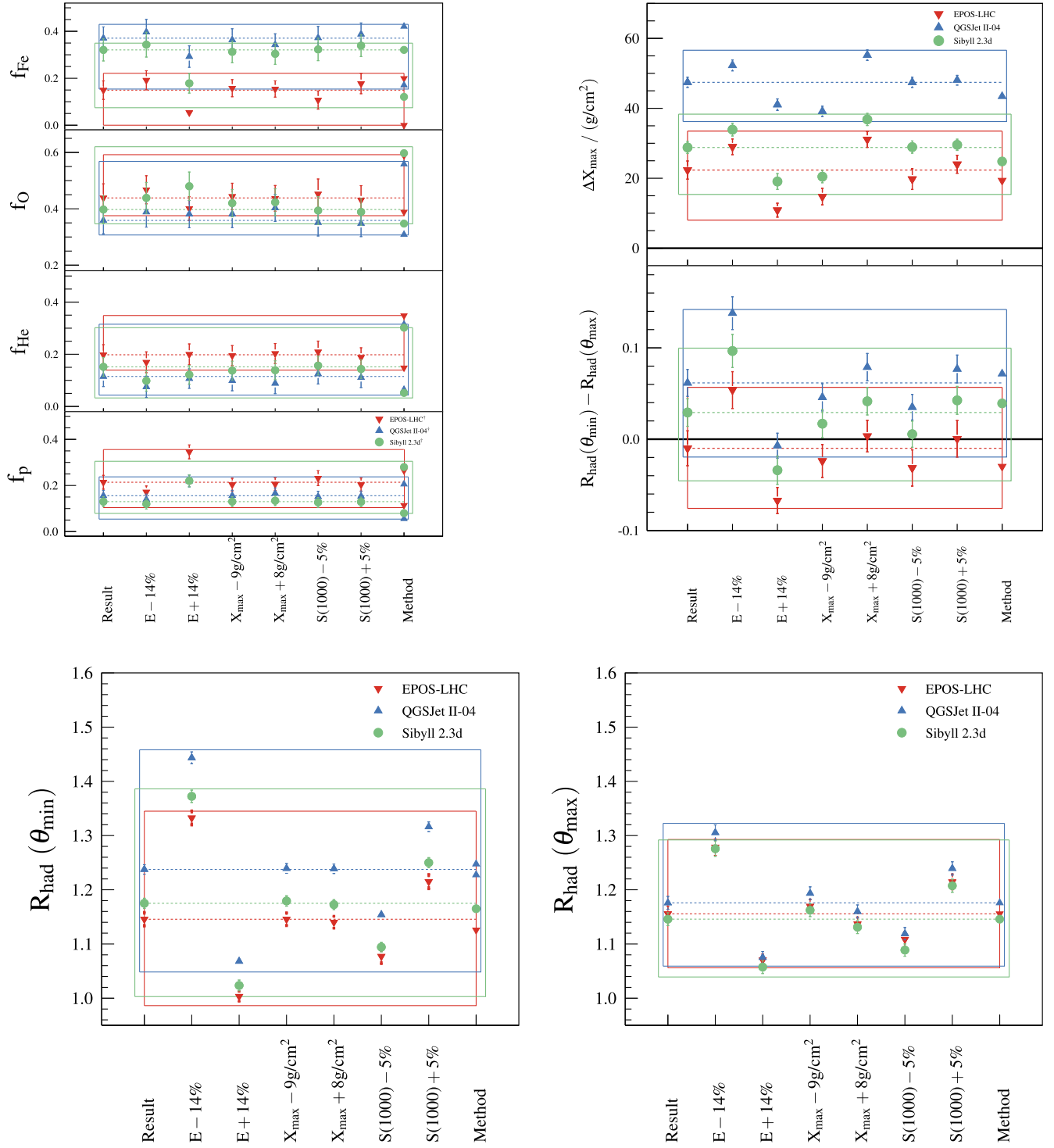
FIG. 16. Contributions of individual experimental systematic uncertainties on energy, X_{\text{max}} , S(1000) and of the method biases inferred from the MC-MC tests (see Appendix B) to the total systematic uncertainties on fractions of primary nuclei (top left), \Delta X_{\text{max}} (top right), R_{\text{had}}(\theta) (bottom) and zenith-angle difference of R_{\text{had}} (top right). Colored bands are the total systematic uncertainties obtained by summing individual contributions in quadrature with the best-fit results indicated by dashed horizontal lines.
