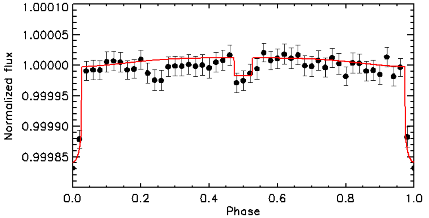
Fig. D.2. TESS binned light curve of HD 20329b (50 bins with a \sim 27 min. bin size), zoomed at the out-of-transit part (phase curve). See details in Appendix D. TLMCM normalized the light curve to phase 0.25.
