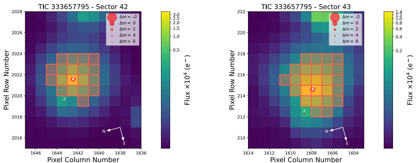
Fig. 1. TESS target pixel file image of HD 20329 observed in sector 42 (left) and sector 43 (right), made with tpfplotter (Aller et al. 2020). The pixels highlighted in red show the aperture used by TESS to create the light curves. The position and sizes of the red circles represent the position and TESS magnitudes of nearby stars, respectively.
