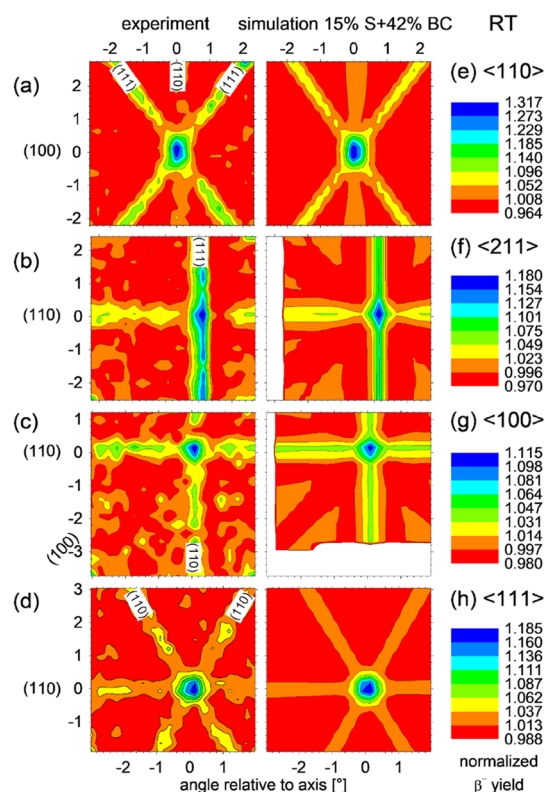
Figure 1. (a–d) Experimental \beta^- EC patterns from 27 Mg in diamond around the \langle 110 \rangle , \langle 211 \rangle , \langle 100 \rangle , and \langle 111 \rangle directions during RT implantation. The panels show the number of detected electrons (normalized intensity indicated by the color scales) as a function of the angle relative to the respective crystal axis. These patterns are a signature for the exact location of the probe atom in the diamond lattice. The plots (e–h) are simulated theoretical patterns considering 15% on ideal substitutional and 42% on ideal BC sites. Note that during the RT \langle 211 \rangle and \langle 100 \rangle measurements, the sample was not yet oriented in such a way that the calculated patterns [ \pm 3.0^\circ ] cover the whole range of measured angles. The areas in the simulated patterns (f,g) which are not covered, are shown in white.
