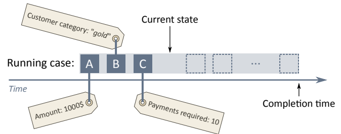
Fig. 1. Graphical representation of the application scenario of the described approach: given a running case we can predict its completion time. We assume that each executed activity (represented as filled boxes) records some additional attributes (represented as labels). Dashed boxes represent future activities.
