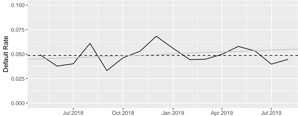
Figure 1: Average (across firms) default rate between May 2018 and August 2019. In grey, the linear regression fit on the default rate.
