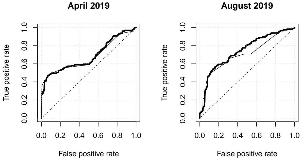
Figure 4: The ROC curves of the CAR model (thick) and the GLM (thin) on the two out-of-sample sets, respectively, April and August 2019. The 45 degree line (dashed) corresponds to random choice.
