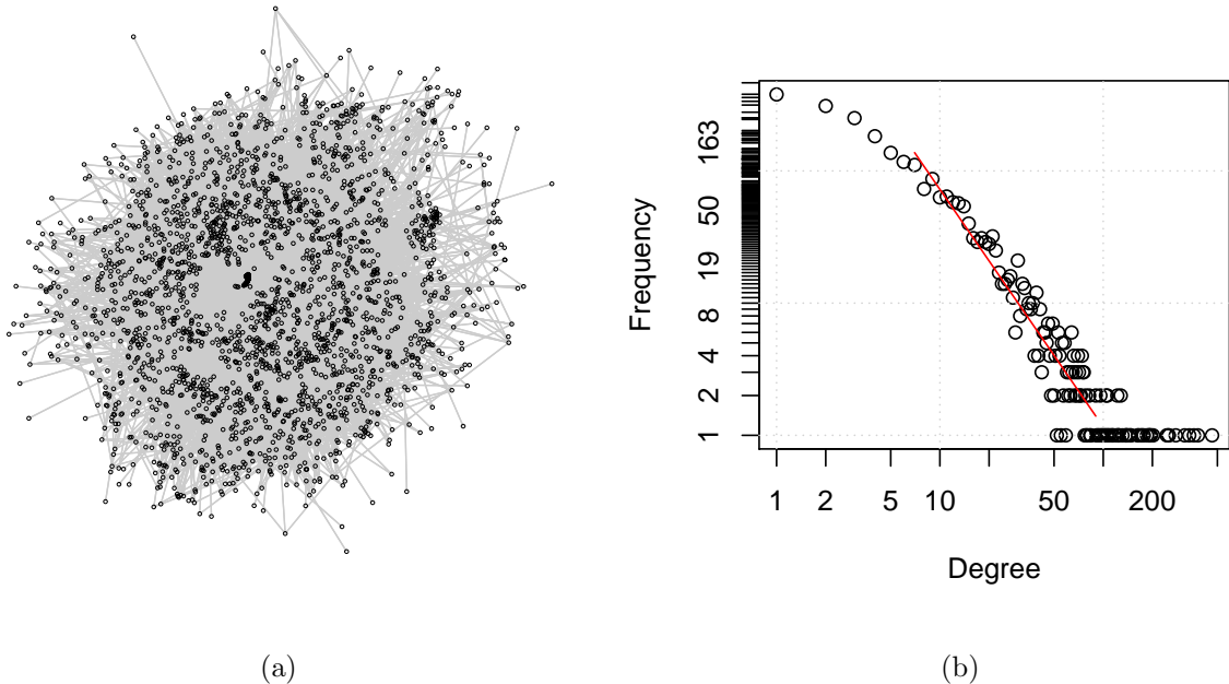
Figure 2: Two representations of the trade network. (a) The biggest connected component of the trade network. A few firms disconnected from this biggest component are omitted for simplicity. (b) Degree distribution of the network. The red line shows a linear regression smoother between the first and third quartiles of the data.
