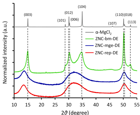
Fig. 2. PXRD patterns of ZNC-bm-DE (green), ZNC-mge-DE (blue), and ZNC-rep-DE (red). All the patterns were extracted from the total scattering data and vertically translated for clarity. The intensity was normalized with the total intensity within the shown 2\theta range. The diffraction pattern of \alpha\text{-MgCl}_2 and the assignment of diffraction planes are also provided as reference.
