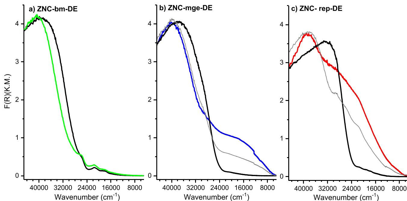
Fig. 6. DR UV-Vis spectra of the three ZN catalysts activated by TEAL: black spectra are the spectra of the pre-catalysts already shown in Fig. 5, green, blue and red spectra are those of the activated catalysts (Al:Ti=2:1), the grey spectra represent an intermediate step in the activation (Al:Ti=1:1) when present.
