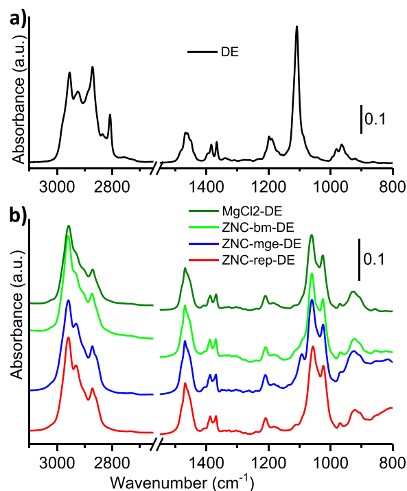
Fig. 4. Part a) ATR-IR spectrum of neat DE. Part b) IR spectra of MgCl 2 -DE (dark green), ZNC-bm-DE (green), ZNC-mge-DE (blue) and ZNC-rep-DE (red), all collected in transmission mode after diluting the samples in KBr. The spectra are vertically translated for clarity.
