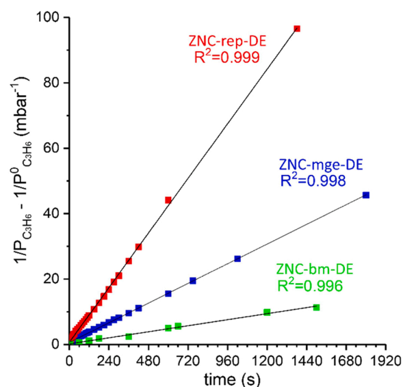
Fig. 8. Kinetics of propylene polymerization on the three catalysts activated by TEAL with an Al:Ti ratio of 2:1. The experimental data (dots) are plotted in terms of reciprocal of monomer pressure (after subtraction of the initial pressure reciprocal) as a function of time and fitted according to second order kinetic law (lines). The goodness of the fit is also reported.
