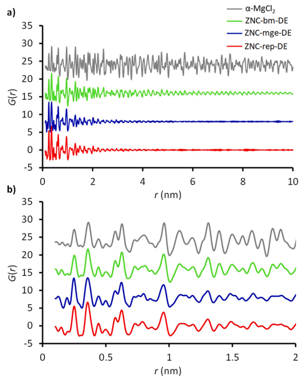
Fig. 3. Part a) PDF patterns of ZNC-bm-DE (green), ZNC-mge-DE (blue), ZNC-rep-DE (red), and \alpha\text{-MgCl}_2 for reference (gray). Part b) the magnified patterns up to r = 2 \text{ nm} . All the patterns were vertically translated in for clarity.
