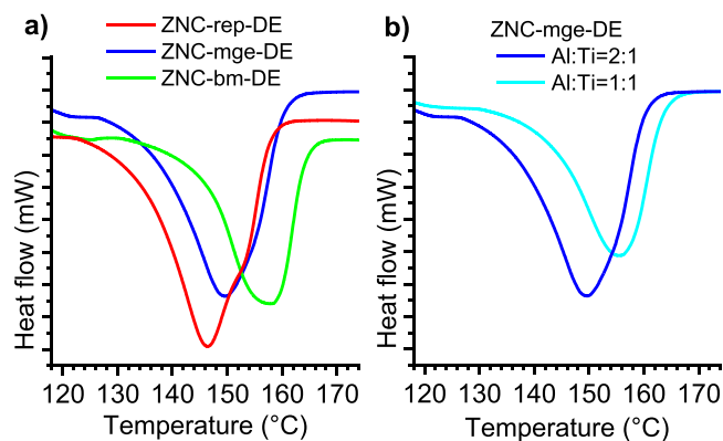
Fig. 9. Part a) DSC profiles of the polymers produced upon the propylene polymerization reactions reported in Fig. 8 (Al:Ti=2:1). Part b) Comparison between the DSC profiles of PP produced by ZNC-mge-DE activated by different amounts of TEAL (either Al:Ti=2:1 or Al:Ti=1:1).
