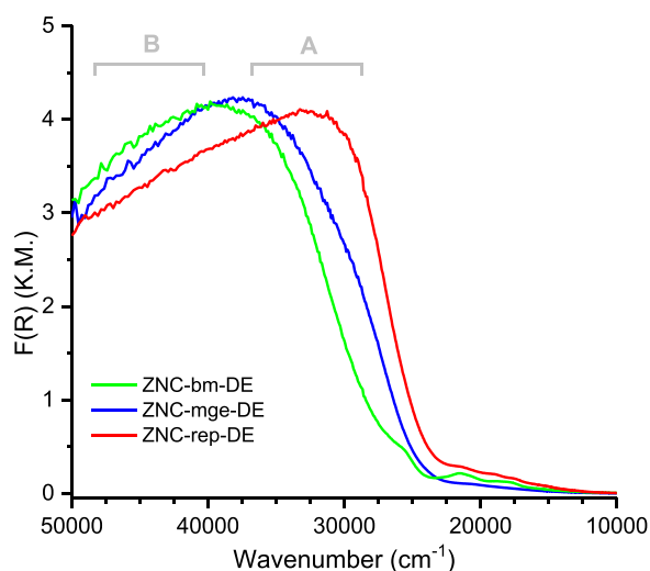
Fig. 5. DR UV-Vis spectra of ZNC-bm-DE (green), ZNC-mge-DE (blue) and ZNC-rep-DE (red). The position of bands of type A and B was determined as the maximum of the second derivative curves, not shown for simplicity.
