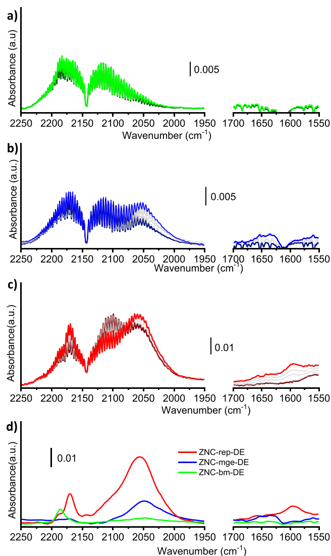
Fig. 7. IR spectra of CO adsorbed at room temperature on activated ZNC-bm-DE (a), ZNC-mge-DE (b) and ZNC-rep-DE (c). In all the sequences, black spectra were collected just after CO dosage, while green, red and blue spectra after 60 min of interaction with CO; grey spectra were collected in between to show the evolution. Part d) Comparison of the three spectra collected after 60 min of interaction with CO, after normalizing the intensities to the optical thickness of the samples and subtracting the roto-vibrational features of CO gas.
