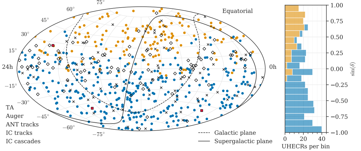
Figure 1. Left: Skymap of the arrival directions of UHECR events and high-energy neutrinos. The high-energy neutrino track-like events from IceCube consists of the HESE, HENU and EHE data sets, while the cascade-like events are only of the IceCube-HESE data sets. From ANTARES, only high-energy tracks are selected for the analyses. Right: A histogram of the declination of UHECR events, separated into Auger and TA contribution.
