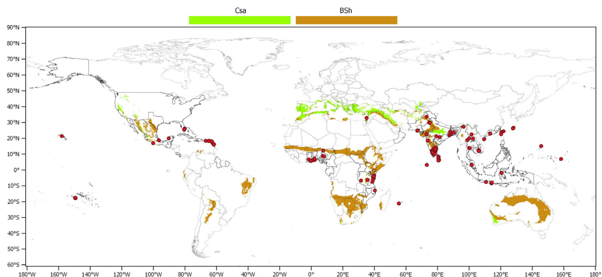
Figure 3: World distribution of selected Köppen–Geiger climate types which occur in the EU and in countries where Paracoccus marginatus has been reported. Red dots indicate point locations of P. marginatus for which geographical coordinates are available
