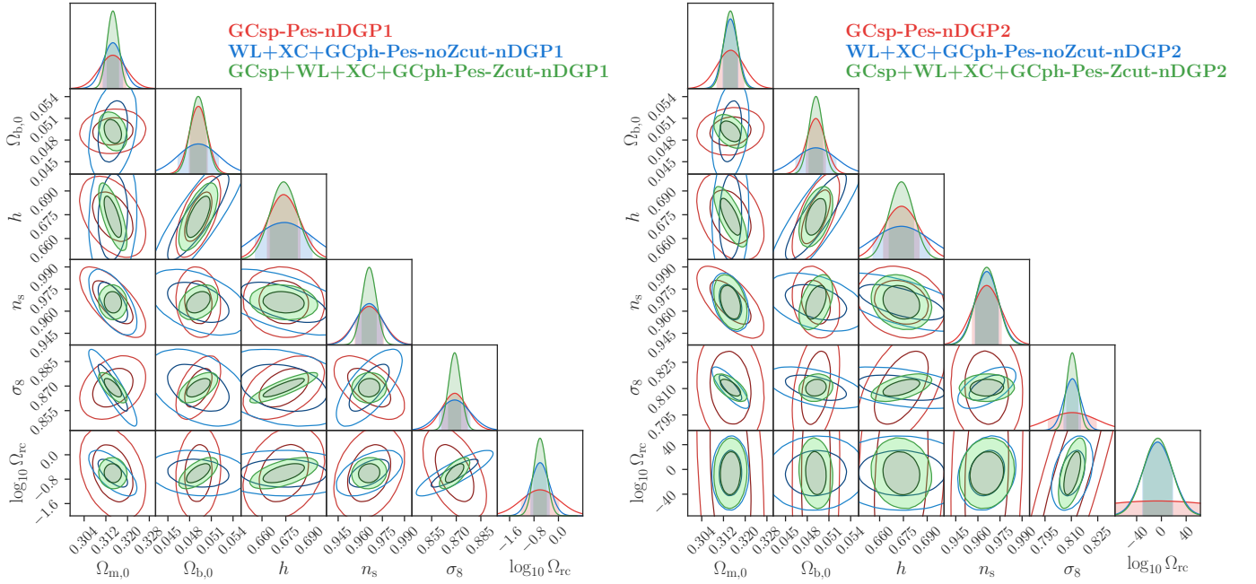
Fig. A.2. 68.3% and 95.4% joint marginal error contours on the cosmological parameters for nDGP1 (left panel) and nDGP2 (right panel) in the pessimistic case. In red, we plot \text{GC}_{\text{sp}} , in blue, we plot \text{WL}+\text{XC}+\text{GC}_{\text{ph}} and in green, we plot \text{GC}_{\text{sp}}+\text{WL}+\text{XC}+\text{GC}_{\text{ph}} .
