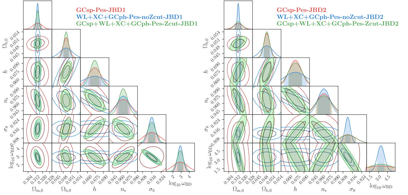
Fig. A.1. 68.3% and 95.4% joint marginal error contours on the cosmological parameters for JBD1 (left panel) and JBD2 (right panel) in the pessimistic case. In red, we plot \text{GC}_{\text{sp}} , in blue, we plot \text{WL}+\text{XC}+\text{GC}_{\text{ph}} and in green, we plot \text{GC}_{\text{sp}}+\text{WL}+\text{XC}+\text{GC}_{\text{ph}} .
