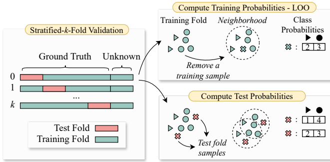
Fig. 2: Overview of the validation methodology for ML stacking. Green indicates training fold samples, red indicates test fold samples and different shapes indicate different classes.
