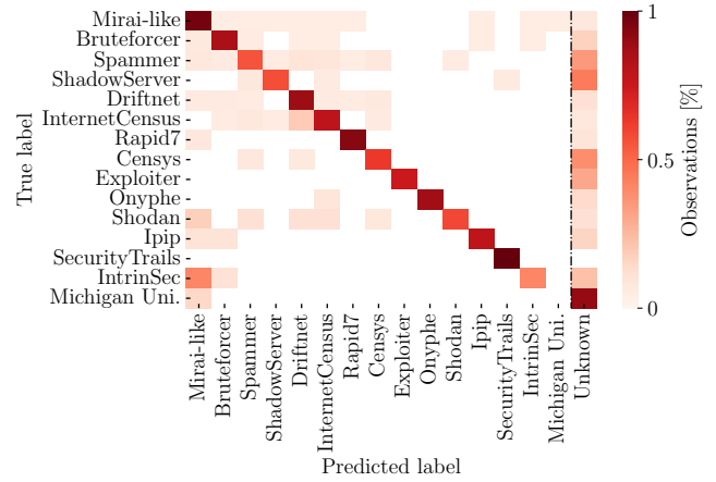
(a) Base model trained on graph embeddings.
