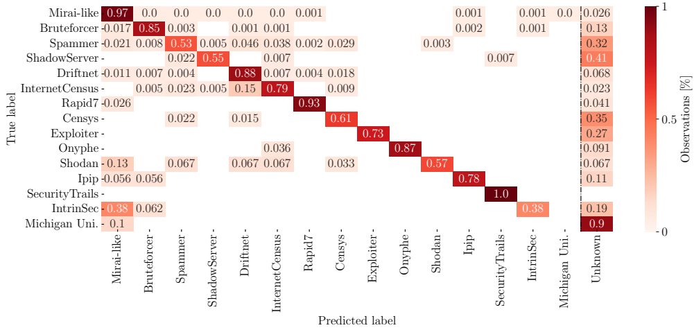
(a) Base model trained on graph embeddings.
