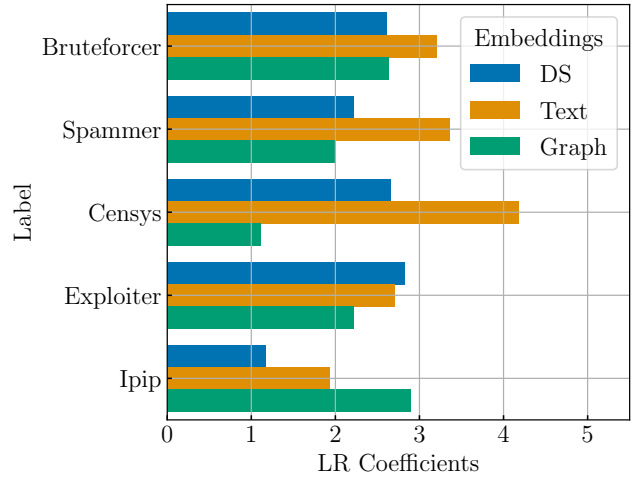
(a) Contribution of different baselines (i.e., embedding types) to ML on Honeypot ( H ) – Scenario 2.
