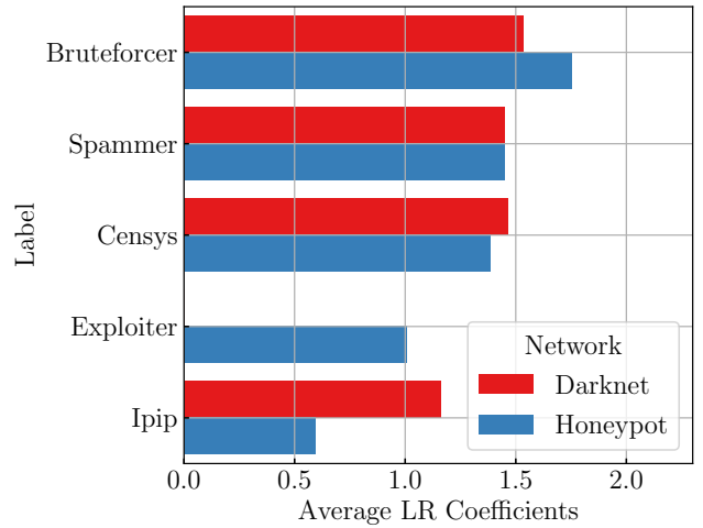
(b) Contribution of different networks on common hosts ( D \cap H ) – Scenario 3.
