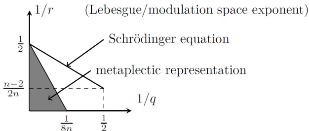
FIGURE 1. Admissible pairs for Strichartz estimates.
