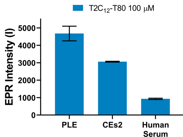
Fig. 6 EPR intensity detected upon 1 h incubation of \text{T2C}_{12} 100 \mu\text{M} + T80 20 \mu\text{M} with PLE, CE2 and human serum at 37^\circ\text{C} under stirring at 400 \text{ rpm} .
