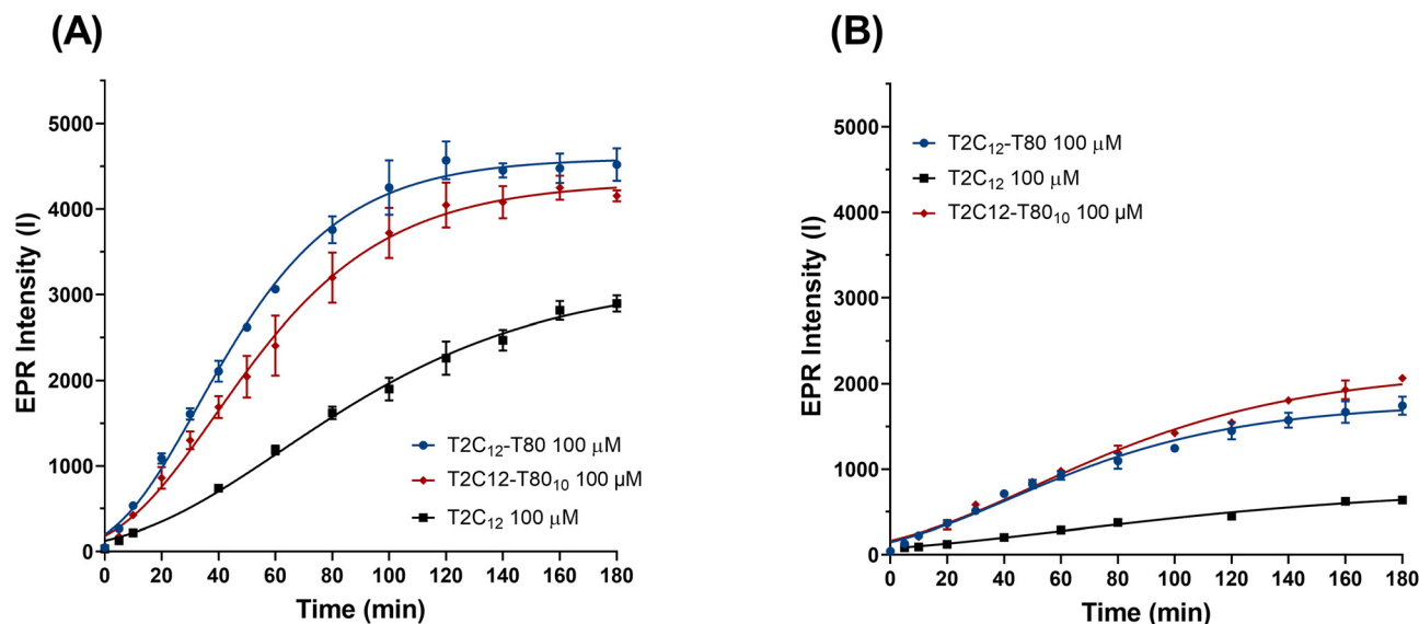
Fig. 4 (A) EPR enzymatic assays with 12 \text{ U mL}^{-1} of CE2 in the presence of \text{T2C}_{12} 100 \mu\text{M} , \text{T2C}_{12}\text{-T80}_{10} 100 \mu\text{M} and \text{T2C}_{12}\text{-T80} 100 \mu\text{M} . (B) Enzymatic assays of \text{T2C}_{12} 100 \mu\text{M} , \text{T2C}_{12}\text{-T80}_{10} 100 \mu\text{M} and \text{T2C}_{12}\text{-T80} 100 \mu\text{M} with CE1 12 \text{ U mL}^{-1} . All kinetics were performed at 37^\circ\text{C} with stirring at 400 \text{ rpm} , and the continuous line was drawn to better show the course of the points.
