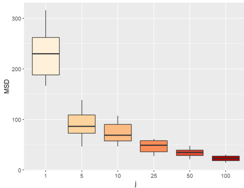
Fig. 6.3 Decrease in variance for different values of j
