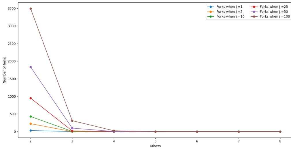
Fig. 6.4 Number of forks involving two or more miners for different values of j
