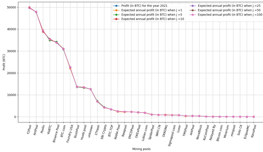
Fig. 6.2 Expected annual profit for different values of j
