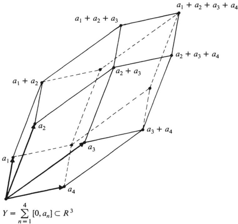
Fig. 1 Zonotope generated by 4 line segments
