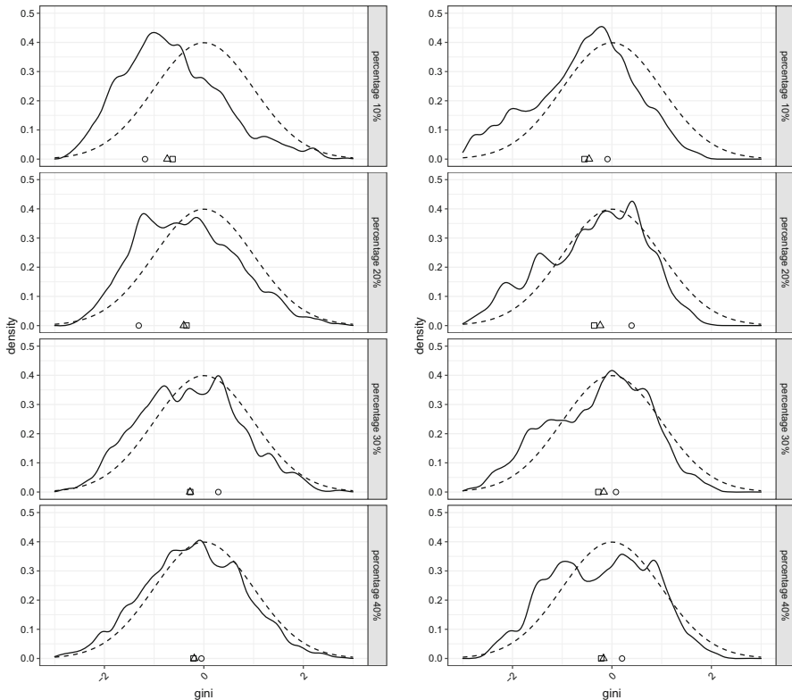
Fig. 3 Kernel distributions of the standard g_j for different sub-sample sizes (solid line) compared with the standard normal distribution (dashed line). The \Delta , \square and \circ represent the mean, median and mode of the distributions of the standard g_j
