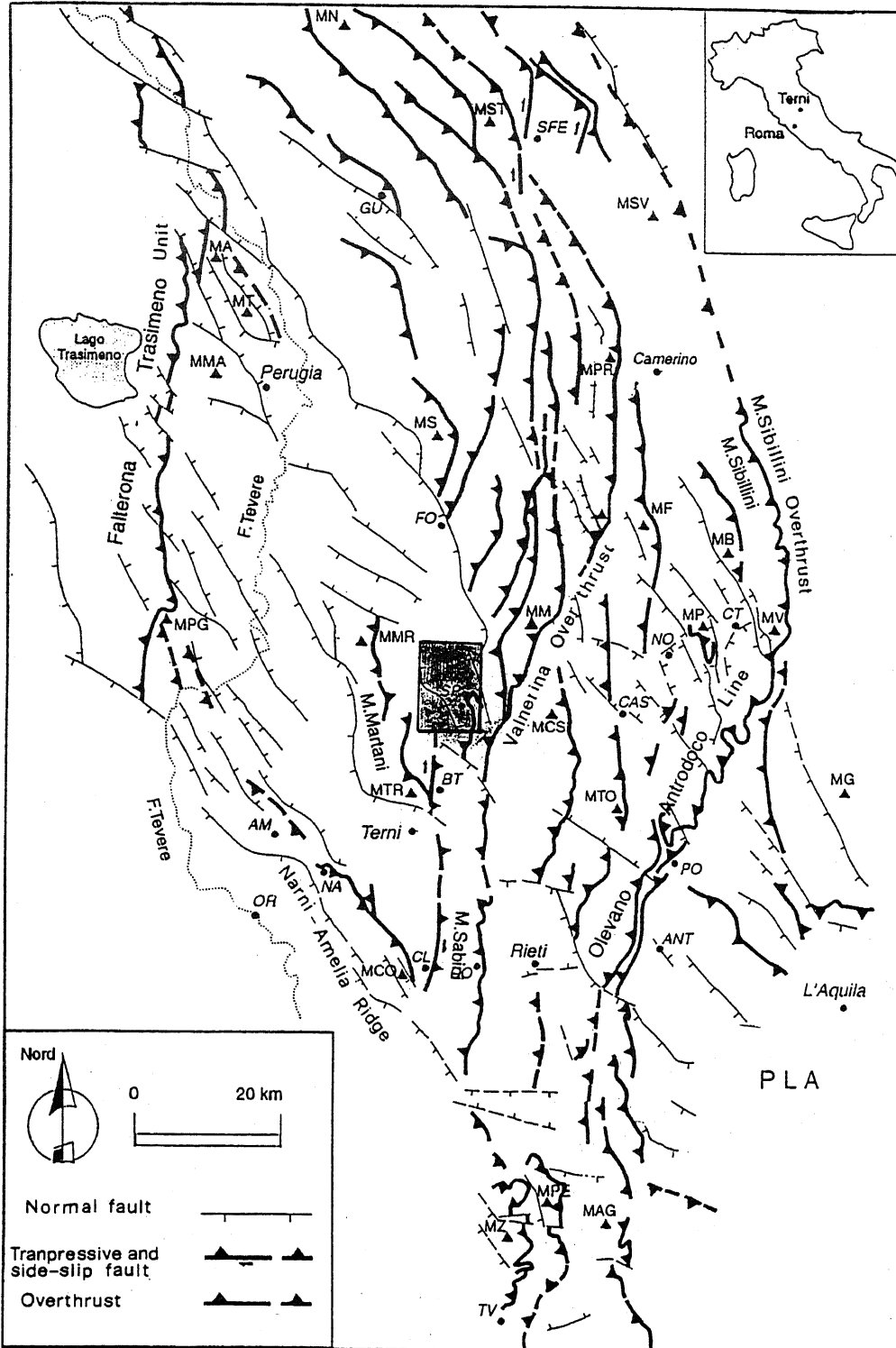
Fig. 1 - Structural setting of the North-central Apennines showing the principal relationships between the Tuscany Domain ( Unità Falterona-Trasimeno ) and the Latium-Abruzzi Platform (PLA) (from Calamita, 1990).
