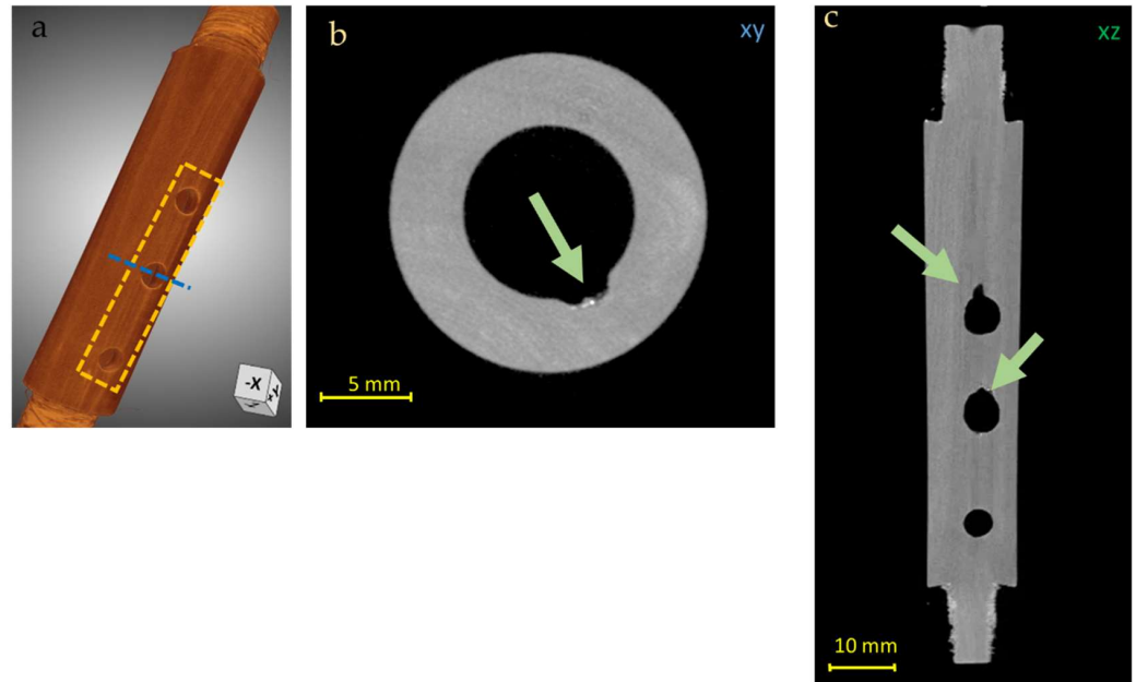
Figure 8. 3D render of the Piccolo Flute body (a) and CT horizontal (b) and vertical (c) slices of the Piccolo Flute body, in which imperfections in the holes are observed (green arrows in (b,c), yellow square in (a)). Blue line in (a) indicates the high of the XY slice (b).
