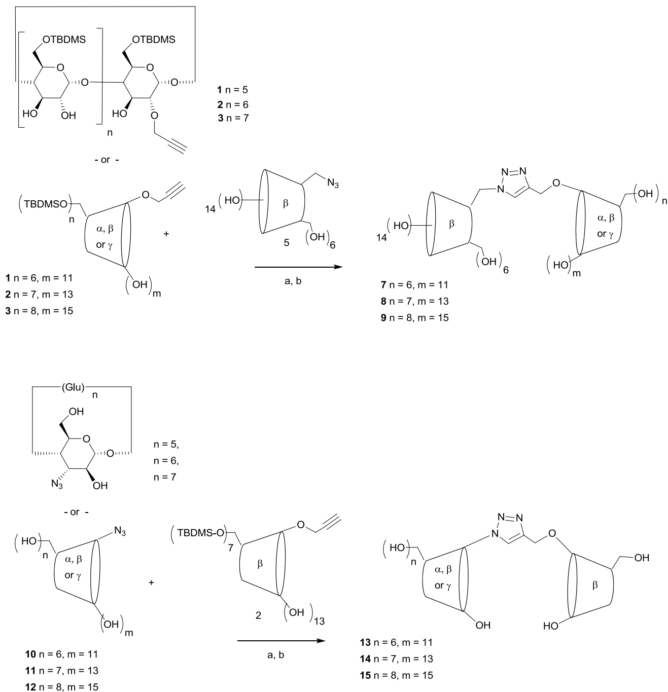
Scheme 3. Synthesis of dimers 7-15 . Reagents and conditions: a ) CuSO_4 /ascorbic acid, t -BuOH/ H_2O (1:1), MW 85^\circ C , 150 W_{max} , 40 min; b ) AcCl 2% in CH_3OH/CH_2Cl_2 1:2
