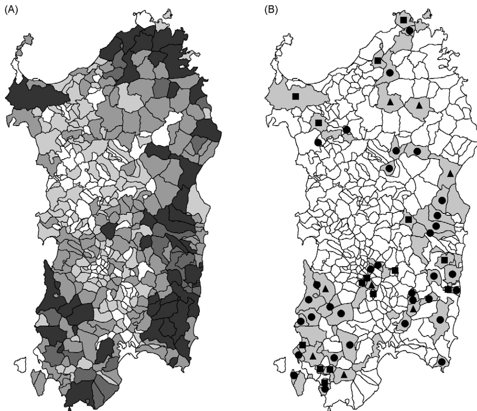
Fig. 1. Map of the Sardinia island, divided in municipalities. (A) Goat herds density. Grey level indicates goat herd density within the municipality: white = less than 1st quartile (3 herds); light grey = between 1st and 2nd quartiles (11 herds); grey = between 2nd and 3rd quartiles (15 herds); dark grey = more than the 3rd quartile. (B) Municipalities including flocks tested with bulk milk analysis (grey). Circles = E positive flocks; squares = B positive flocks; triangles = coinfecting (or uncharacterized) flocks.
