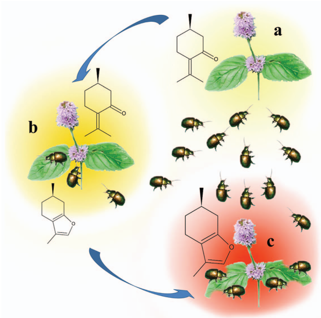
Figure 6. The behavior of C. herbacea and M. aquatica before and during herbivore feeding. a, Undamaged plants emit (+)-pulegone, which acts as an attractant for C. herbacea . b, Feeding activity induces gene expression and increases content of the deterrent compound (+)-menthofuran, along with the emission of the attractant compound (+)-pulegone; as a result, fewer insects are attracted to the plants. c, Intense feeding induces a reduction in (+)-pulegone content and a dramatic increase in the repellent compound (+)-menthofuran; C. herbacea avoids over-fed plants and moves towards undamaged plants. doi:10.1371/journal.pone.0017195.g006
