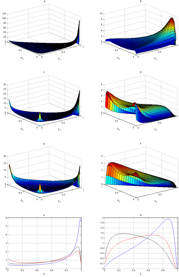
Figure .1: NID distribution based on gamma and inverse-Gaussian r.v.: A) on \Delta^{(2)} with \alpha_1 = 0.5790 , \gamma_1 = 1 , \lambda_i = 0.1667 , \theta_i = 1 , i = 1, 2 . B) on \Delta^{(2)} with \alpha_i = 1.09 , \gamma_1 = 1 , \lambda_i = 0.6 , \theta_i = 1 , i = 1, 2 . C) on \Delta^{(2)} with \alpha_1 = 0.5790 , \gamma_1 = 3 , \lambda_i = 0.1667 , \theta_i = 1 , i = 1, 2 . D) on \Delta^{(2)} with \alpha_1 = 1.09 , \gamma_1 = 3 , \lambda_i = 0.6 , \theta_i = 1 , i = 1, 2 . E) on \Delta^{(2)} with \alpha_i = 0.5790 , \gamma_i = 3 , i = 1, 2 , \lambda_1 = 0.1667 , \theta_1 = 1 . F) on \Delta^{(2)} with \alpha_i = 1.09 , \gamma_i = 3 , i = 1, 2 , \lambda_1 = 0.6 , \theta_1 = 1 . G) on (0, 1) with \alpha_1 = 0.8685 , \lambda_1 = 0.25 , \gamma_1 = 1 , \theta_1 = 1 (blue), \gamma_1 = 3 , \theta_1 = 1 (red) and with \gamma_1 = 3 , \theta_1 = 2 (black). H) on (0, 1) with \alpha_1 = 1.6350 , \lambda_1 = 0.9 , \gamma_1 = 1 , \theta_1 = 1 (blue), \gamma_1 = 2 , \theta_1 = 1 (red) and with \gamma_1 = 3 , \theta_1 = 1 (black).
