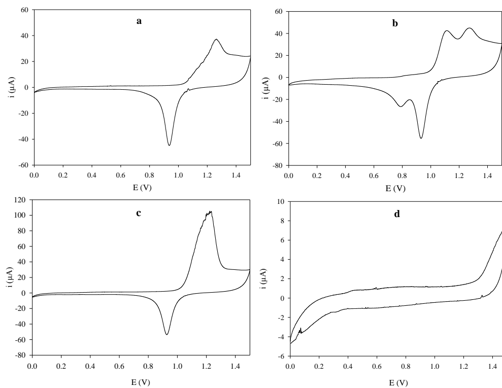
Fig. 1. Cyclic voltammograms obtained in 0.5 M \text{H}_2\text{SO}_4 with the lateral gold electrode for a) a clean surface; b) the surface in the presence of multilayers of oxides; c) the surface after the growth of an important oxide layer; d) the surface covered by a passivating layer.
