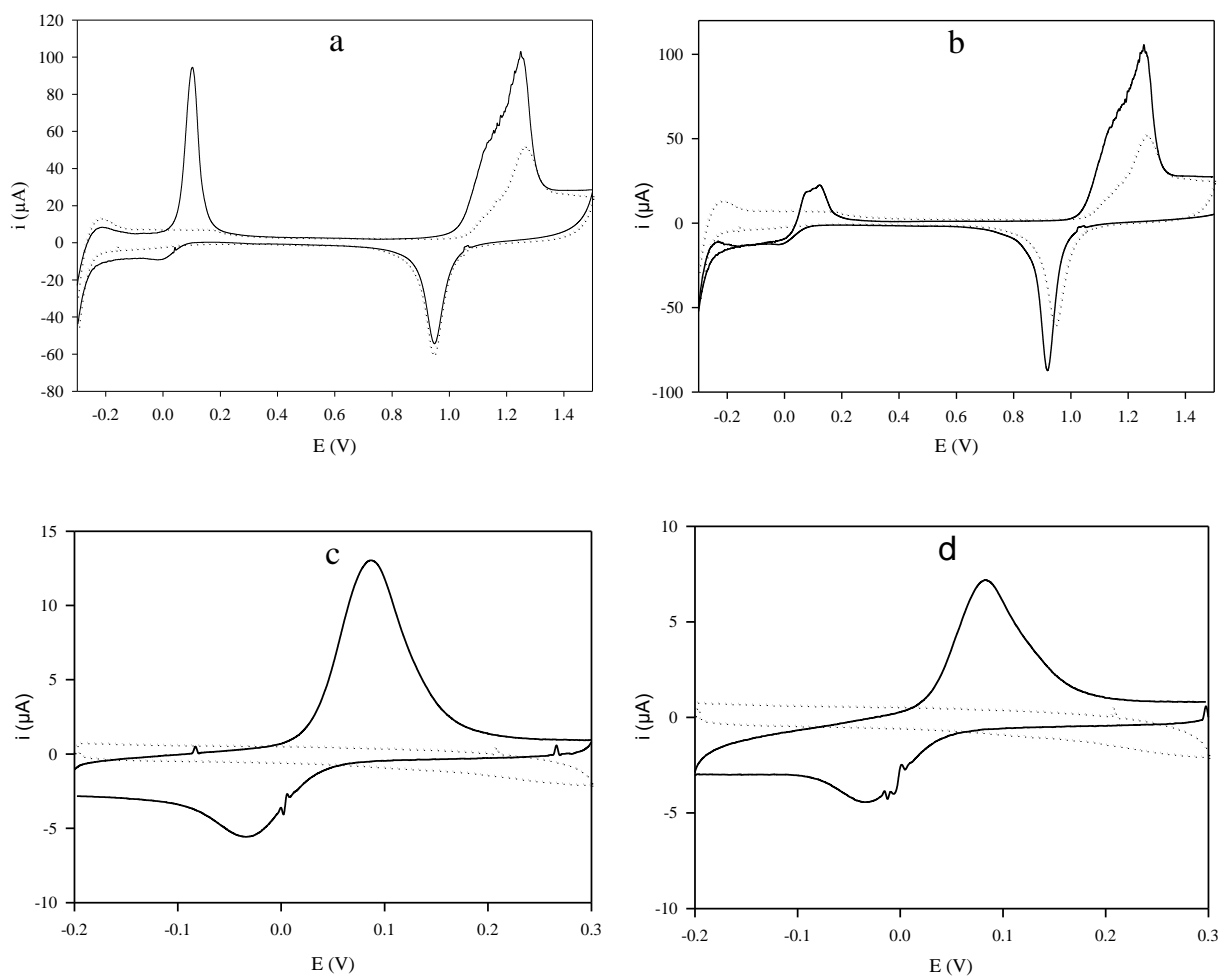
Fig. 6. Voltammograms of blank (····) and of 20 μg l -1 of As(III) (—) obtained working in a) reverse scan in 0.5 M H 2 SO 4 ; b) direct scan in H 2 SO 4 ; c) reverse scan in 0.25 M HCl; d) direct scan in HCl.
