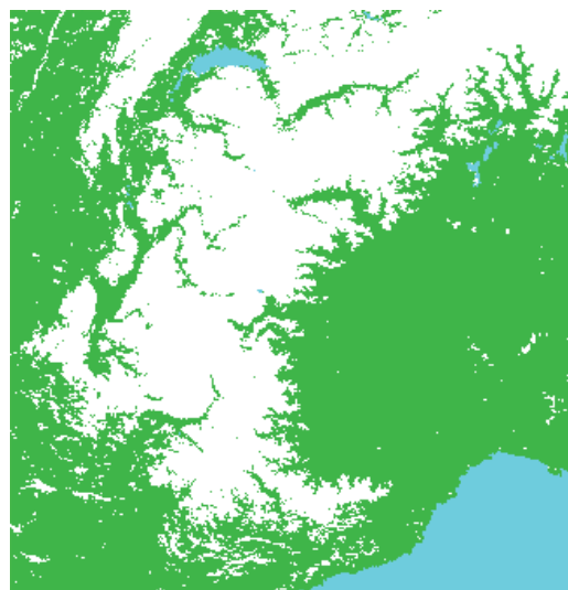
Figure 5. Maximum snow cover in the period 02 February-05 March 2007: snow is represented in white.
