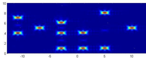
Figure 6: Filtered representation.
