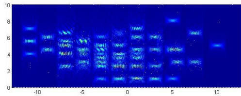
Figure 5: Wig(f)(x, \omega)
