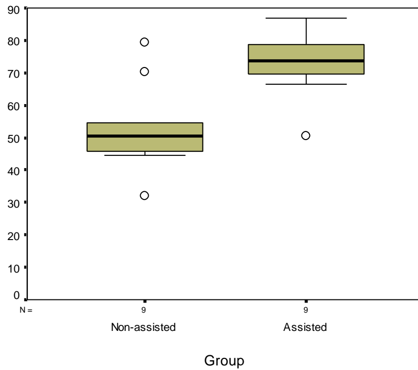
Figure 2. Boxplot of final score for assisted vs. non-assisted group
