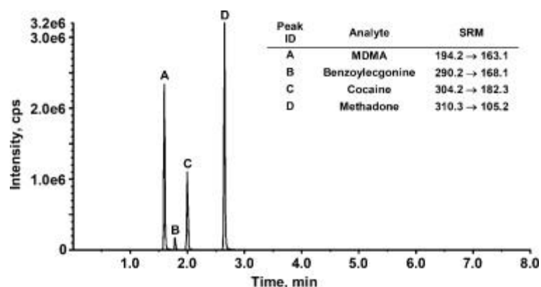
Fig. 2. MRM chromatogram of a real sample positive to MDMA, cocaine, BZE and methadone.
