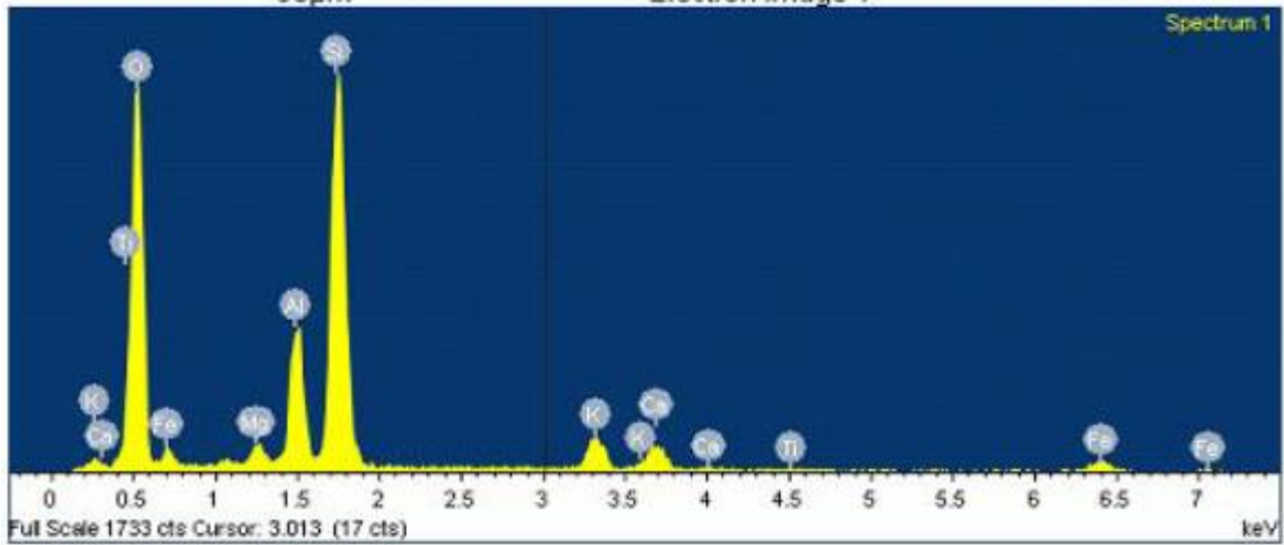
Figure S2. FESEM image and EDX analysis of the zeolite sample.
