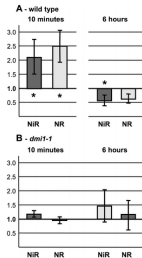
Fig. 5 NiR and NR relative expression in M. truncatula wild-type (a) or dmi1-1 (b) roots exposed to the fungal exudate for 10 min or 6 h. Gene expression was normalized to the MtTefA gene and reported as the amount of induction relative to control roots treated with sterile water. Asterisks indicate statistically significant differences in gene expression levels between roots treated with fungal exudate and roots treated with sterile water ( p < 0.05 , one-way ANOVA and Tukey's post hoc test)
