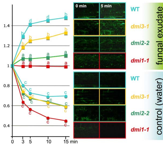
Fig. 3 Time course analysis of DAF-2T fluorescence intensity in wild-type (cyan), dmi1-1 (red), dmi2-2 (green), and dmi3-1 (yellow) M. truncatula ROC at 0, 3, 5, 10, and 15 min after treatment with the fungal exudate (squares) or with sterile water (circles) as control. Values indicate the ratio of fluorescence intensity at each time point to the respective intensity at time 0. Different letters indicate statistically significant differences ( p < 0.05 , Kruskal–Wallis test). Images of fluorescence at time 0 and after 5 min are shown on the right.
