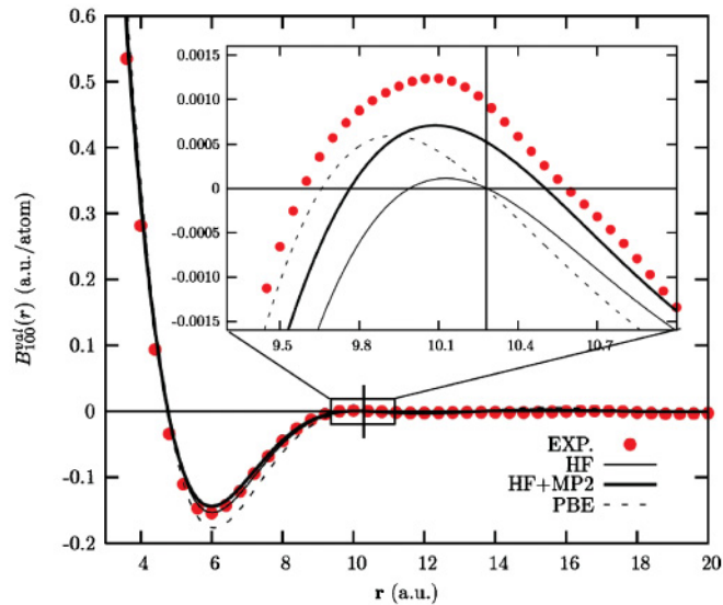
FIG. 5. (Color online) Theoretical and experimental valence AFs along the [100] crystallographic direction. Symbols as in Fig. 4. These plots partially coincide with those reported in Ref. 18.
