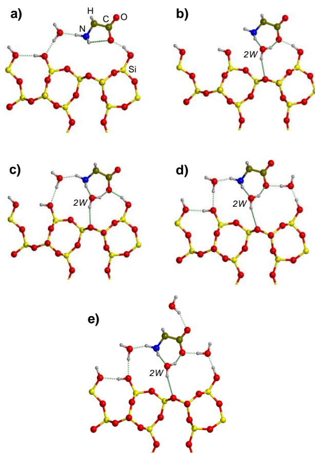
Figure 69. The most stable structures found in Ref. 322 for the successive addition of water (from 1 to 5, a–e, respectively) at the Gly-zwitter/silica surface interface. Periodic systems optimized at the B3LYP/triple- \zeta level. Adapted with permission from Ref. 322 . Copyright 2008 American Chemical Society.
