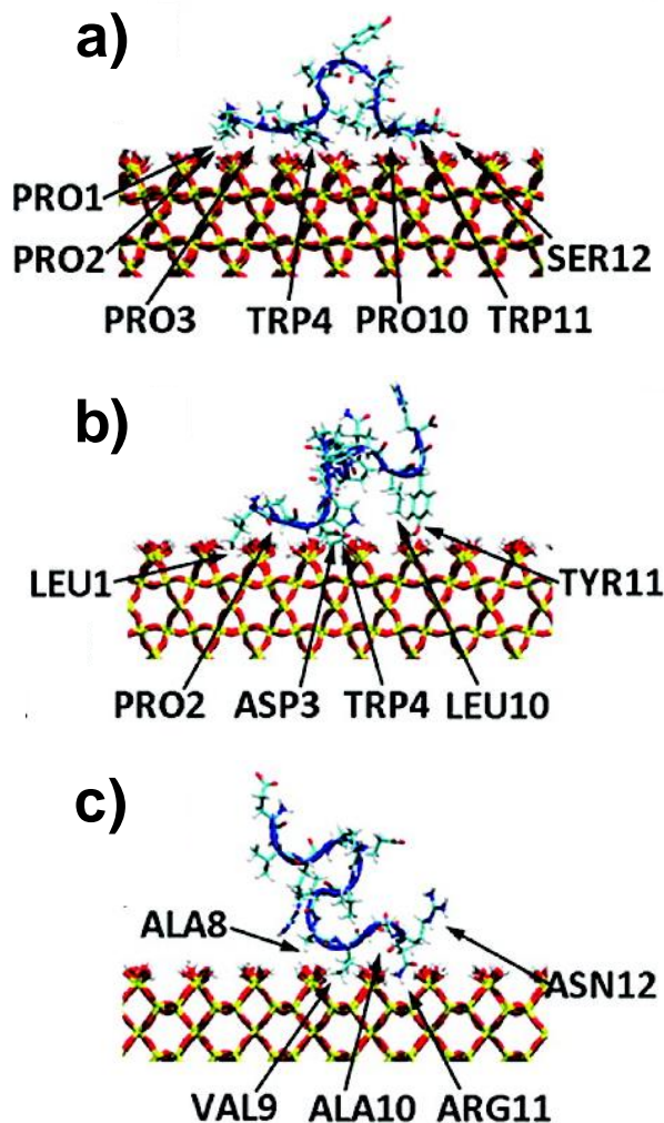
Figure 84. Snapshots of the peptide/silica systems during classical MD simulations in aqueous solvent (CHARMM-type force field, T = 300\text{K} ), of the for strong-binding peptides (a and b) and the weak-binding peptide (c). Water molecules have been omitted for the sake of clarity. Adapted with permission from Ref. 272 . Copyright 2010 American Chemical Society.
