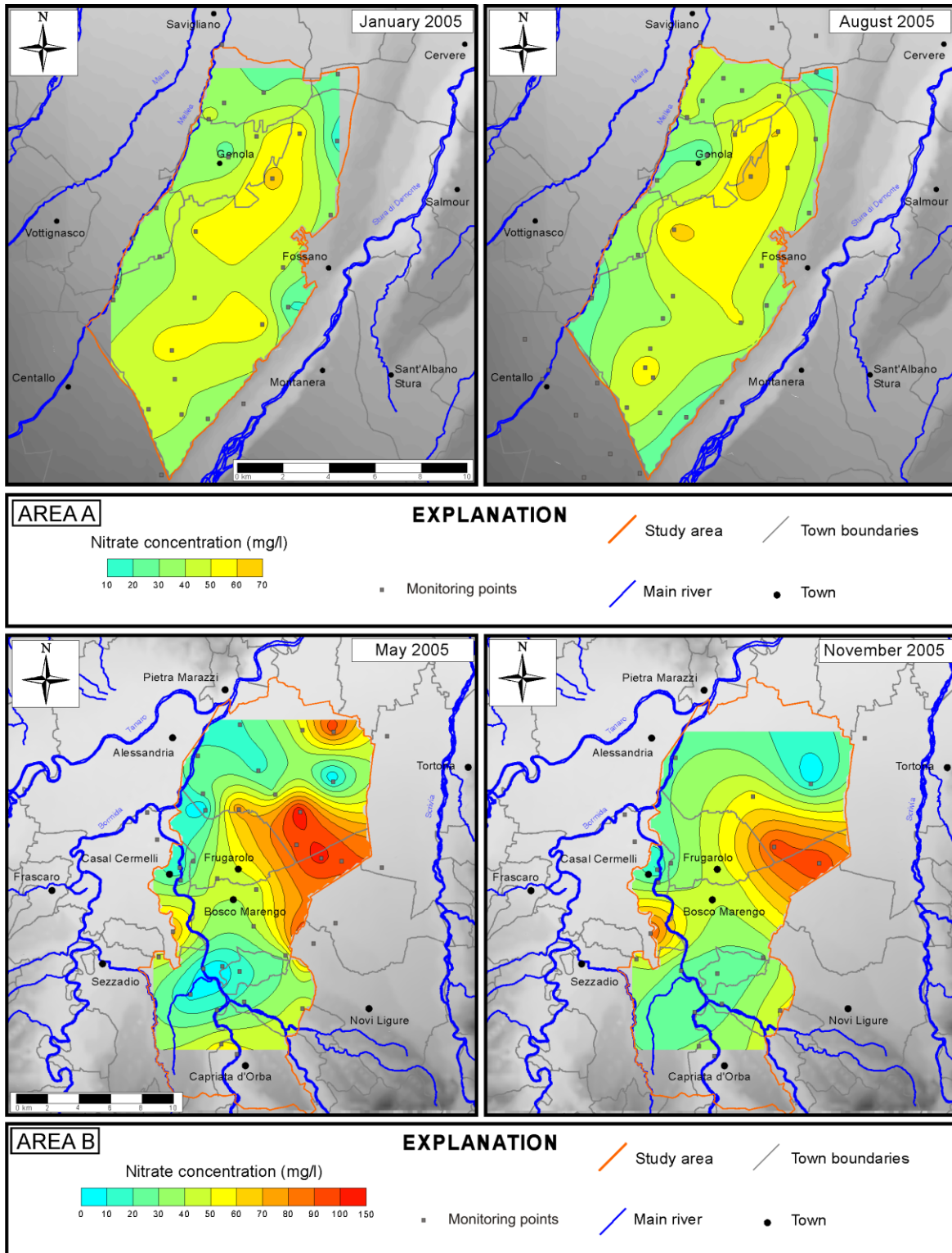
Fig. 8: Nitrate concentration maps in Area A (January 2005 and August 2005) and in Area B (May 2005 and November 2005).
