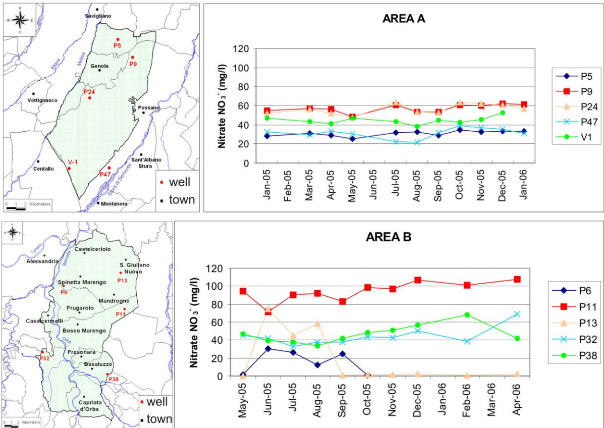
Fig. 9: Time series of observed NO 3 - concentration of five monitoring wells in Study Area A and in Study Area B, and their location.
