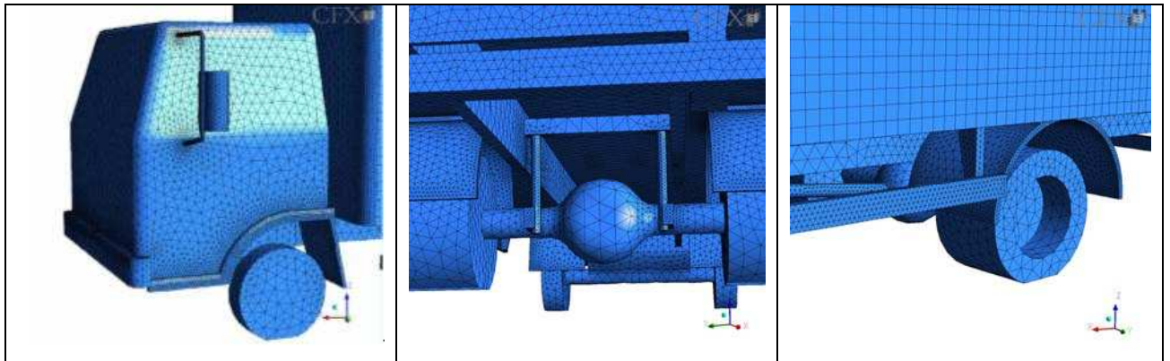
Fig. 4 : Details of the surface mesh for CFD computations
