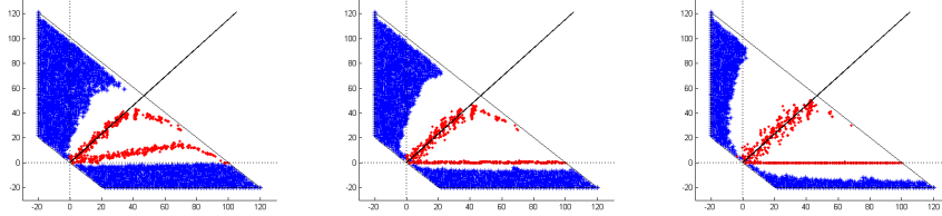
Figure 4: Transaction region in the plane (B, S) . Time t = 0.5 (left) - t = 0.75 (middle) - t = 0.9 (right), N = 5000 , W = 250 , K = 0.1 and c = 0.01 .
